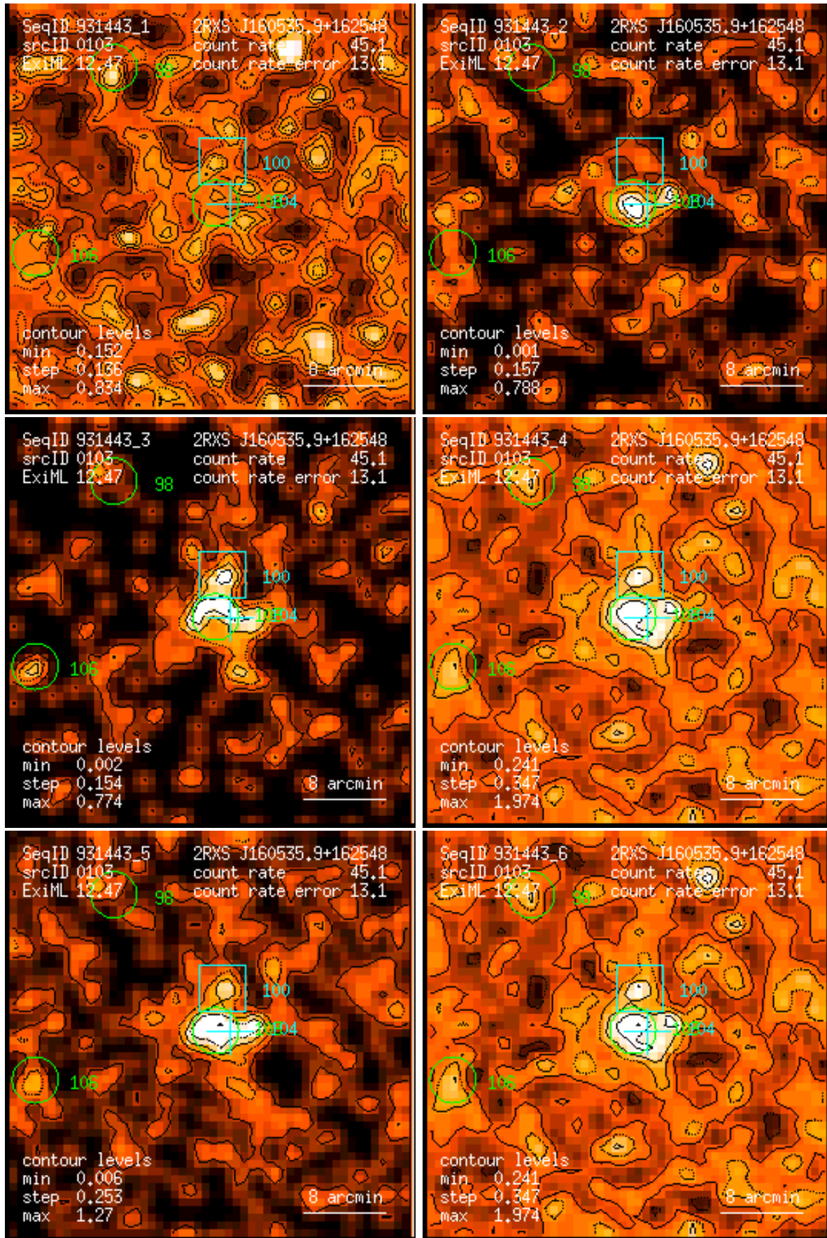
Figure 103: RASS 931443: detection 0103: band rate images, Gaussian filter: (1) PSPC channels 11 – 41, (2) 52 – 90, (3) 91 – 201, (4) 11 – 235, (5) 52 – 201, (6) 11 – 201. Broad band rates in counts/ks. Band rate contour levels in counts/ks/arcmin 2 .
