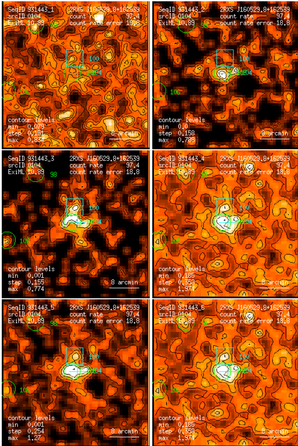
Figure 104: RASS 931443: detection 0104: band rate images, Gaussian filter: (1) PSPC channels 11 – 41, (2) 52 – 90, (3) 91 – 201, (4) 11 – 235, (5) 52 – 201, (6) 11 – 201. Broad band rates in counts/ks. Band rate contour levels in counts/ks/arcmin 2 .
