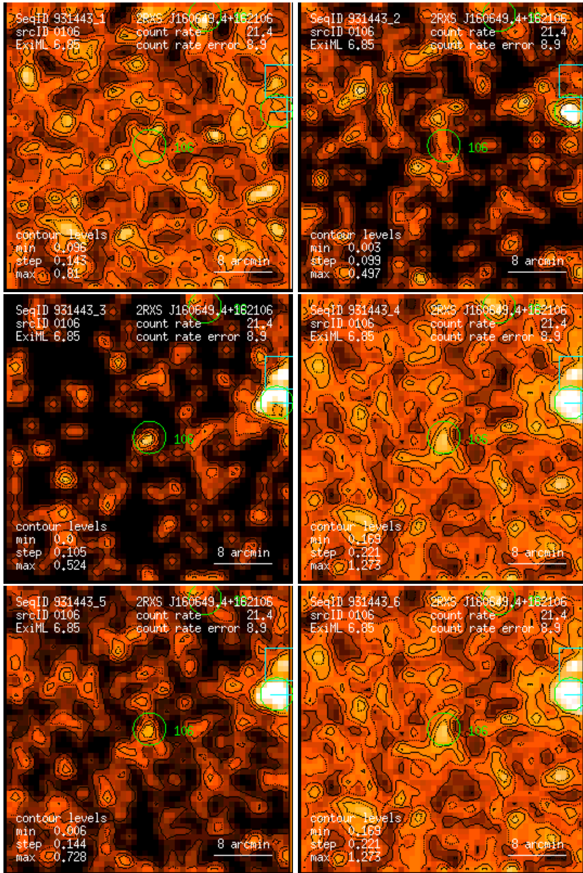
Figure 106: RASS 931443: detection 0106: band rate images, Gaussian filter: (1) PSPC channels 11 – 41, (2) 52 – 90, (3) 91 – 201, (4) 11 – 235, (5) 52 – 201, (6) 11 – 201. Broad band rates in counts/ks. Band rate contour levels in counts/ks/arcmin 2 .
