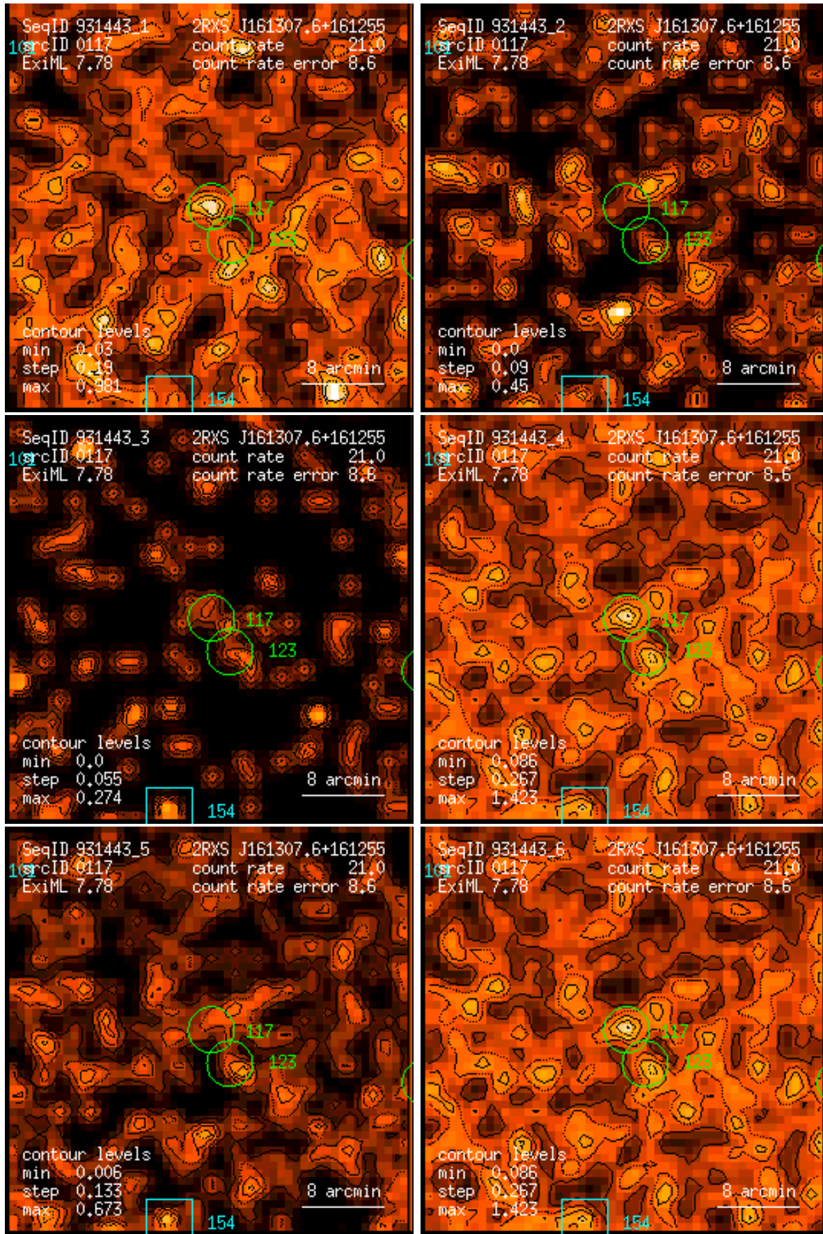
Figure 117: RASS 931443: detection 0117: band rate images, Gaussian filter: (1) PSPC channels 11 – 41, (2) 52 – 90, (3) 91 – 201, (4) 11 – 235, (5) 52 – 201, (6) 11 – 201. Broad band rates in counts/ks. Band rate contour levels in counts/ks/arcmin 2 .
