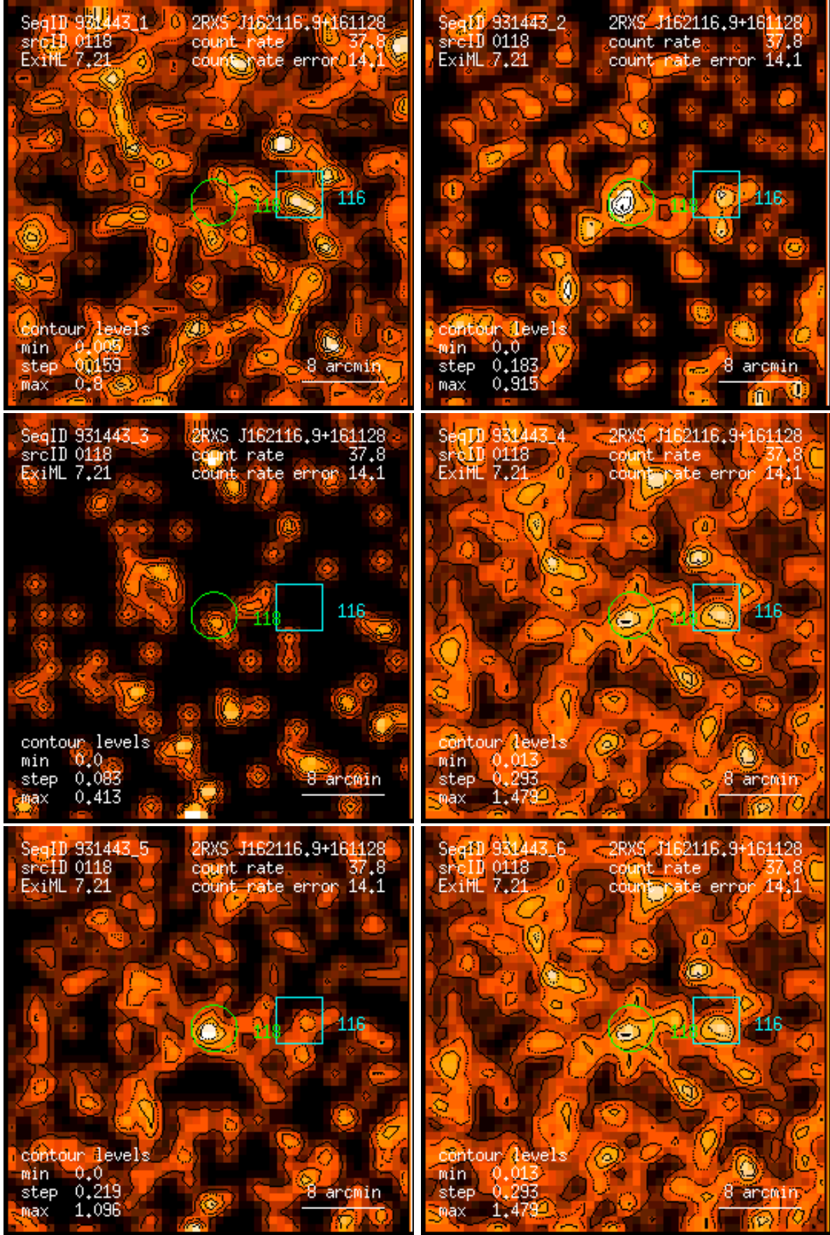
Figure 118: RASS 931443: detection 0118: band rate images, Gaussian filter: (1) PSPC channels 11 – 41, (2) 52 – 90, (3) 91 – 201, (4) 11 – 235, (5) 52 – 201, (6) 11 – 201. Broad band rates in counts/ks. Band rate contour levels in counts/ks/arcmin 2 .
