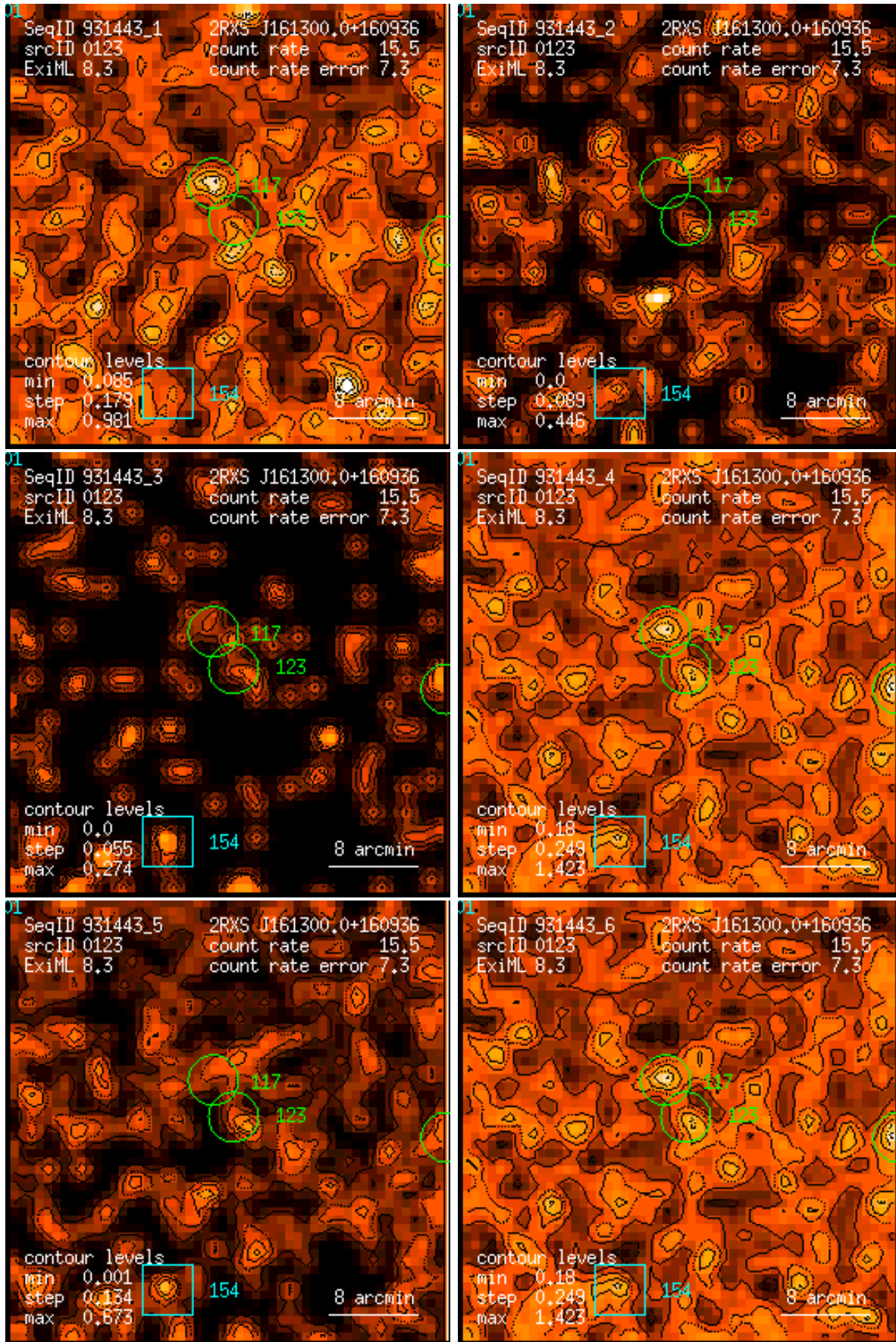
Figure 123: RASS 931443: detection 0123: band rate images, Gaussian filter: (1) PSPC channels 11 – 41, (2) 52 – 90, (3) 91 – 201, (4) 11 – 235, (5) 52 – 201, (6) 11 – 201. Broad band rates in counts/ks. Band rate contour levels in counts/ks/arcmin 2 .
