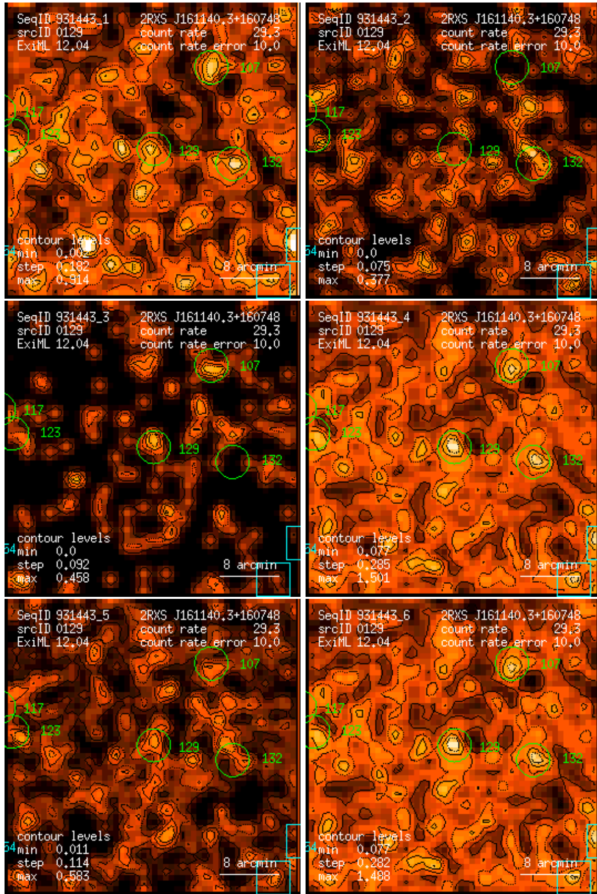
Figure 129: RASS 931443: detection 0129: band rate images, Gaussian filter: (1) PSPC channels 11 – 41, (2) 52 – 90, (3) 91 – 201, (4) 11 – 235, (5) 52 – 201, (6) 11 – 201. Broad band rates in counts/ks. Band rate contour levels in counts/ks/arcmin 2 .
