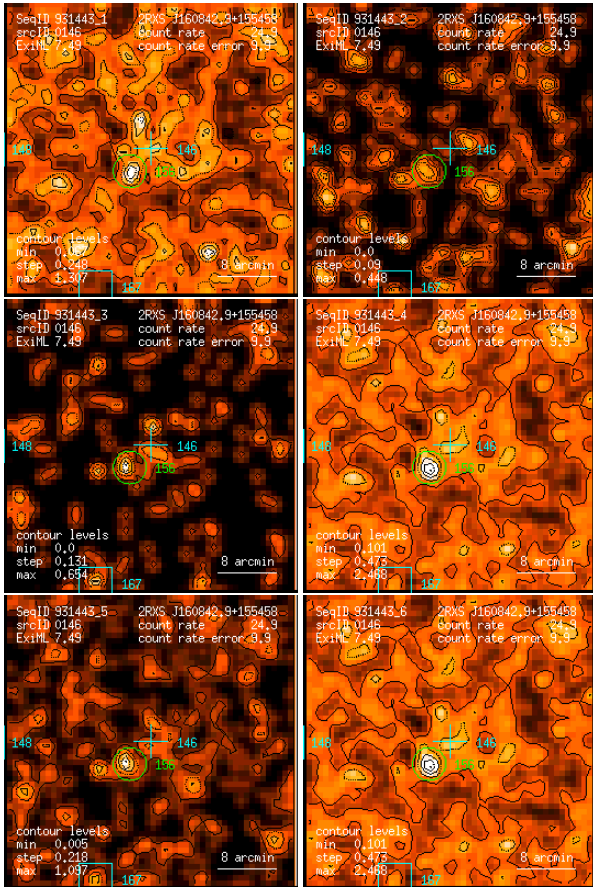
Figure 146: RASS 931443: detection 0146: band rate images, Gaussian filter: (1) PSPC channels 11 – 41, (2) 52 – 90, (3) 91 – 201, (4) 11 – 235, (5) 52 – 201, (6) 11 – 201. Broad band rates in counts/ks. Band rate contour levels in counts/ks/arcmin 2 .
