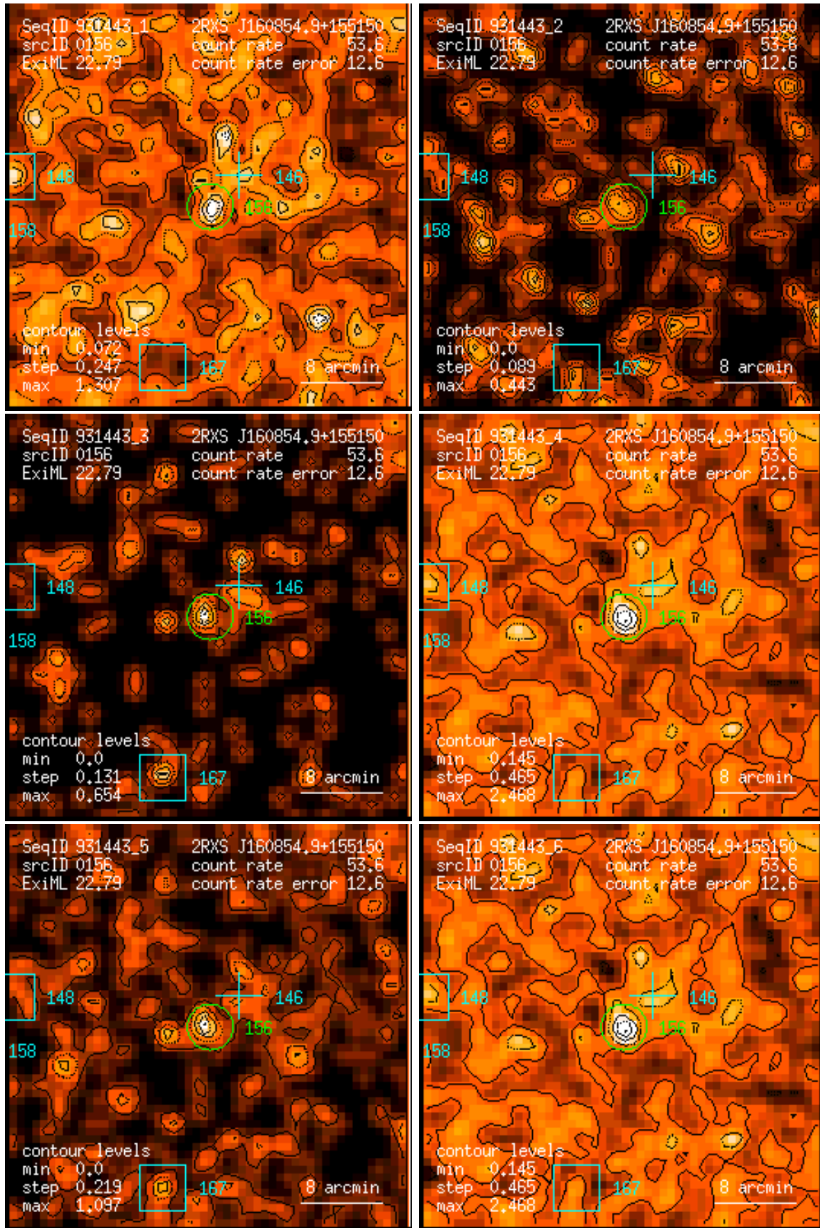
Figure 156: RASS 931443: detection 0156: band rate images, Gaussian filter: (1) PSPC channels 11 – 41, (2) 52 – 90, (3) 91 – 201, (4) 11 – 235, (5) 52 – 201, (6) 11 – 201. Broad band rates in counts/ks. Band rate contour levels in counts/ks/arcmin 2 .
