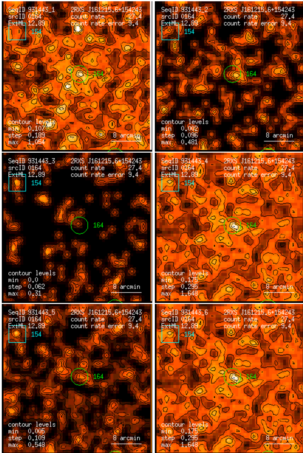
Figure 164: RASS 931443: detection 0164: band rate images, Gaussian filter: (1) PSPC channels 11 – 41, (2) 52 – 90, (3) 91 – 201, (4) 11 – 235, (5) 52 – 201, (6) 11 – 201. Broad band rates in counts/ks. Band rate contour levels in counts/ks/arcmin 2 .
