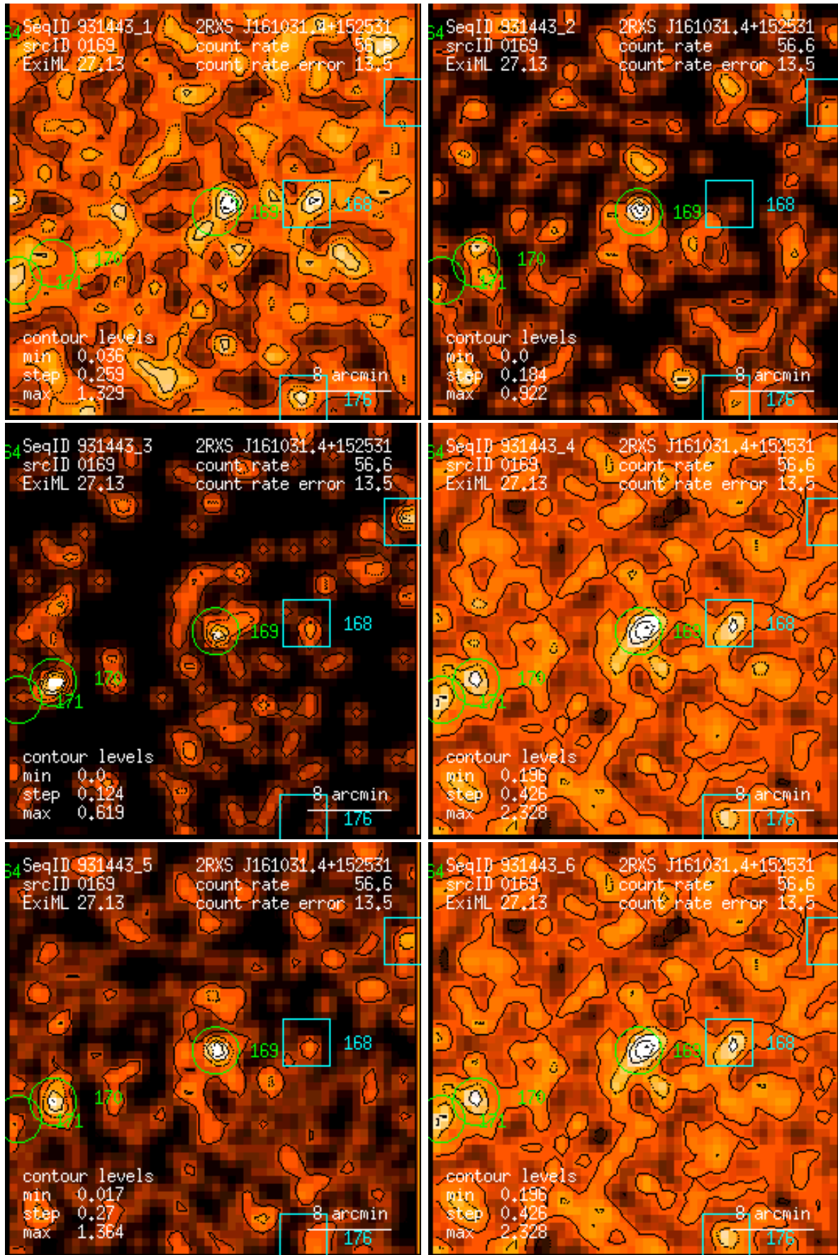
Figure 169: RASS 931443: detection 0169: band rate images, Gaussian filter: (1) PSPC channels 11 – 41, (2) 52 – 90, (3) 91 – 201, (4) 11 – 235, (5) 52 – 201, (6) 11 – 201. Broad band rates in counts/ks. Band rate contour levels in counts/ks/arcmin 2 .
