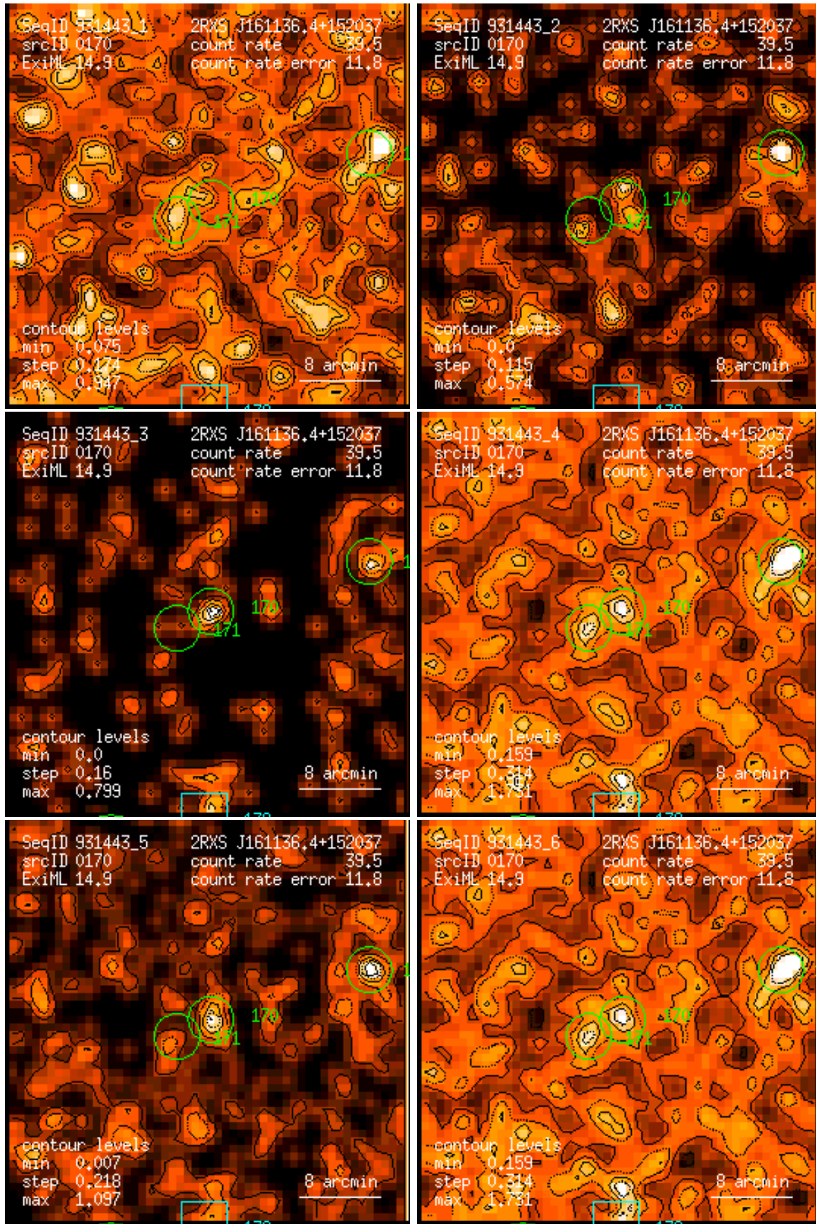
Figure 170: RASS 931443: detection 0170: band rate images, Gaussian filter: (1) PSPC channels 11 – 41, (2) 52 – 90, (3) 91 – 201, (4) 11 – 235, (5) 52 – 201, (6) 11 – 201. Broad band rates in counts/ks. Band rate contour levels in counts/ks/arcmin 2 .
