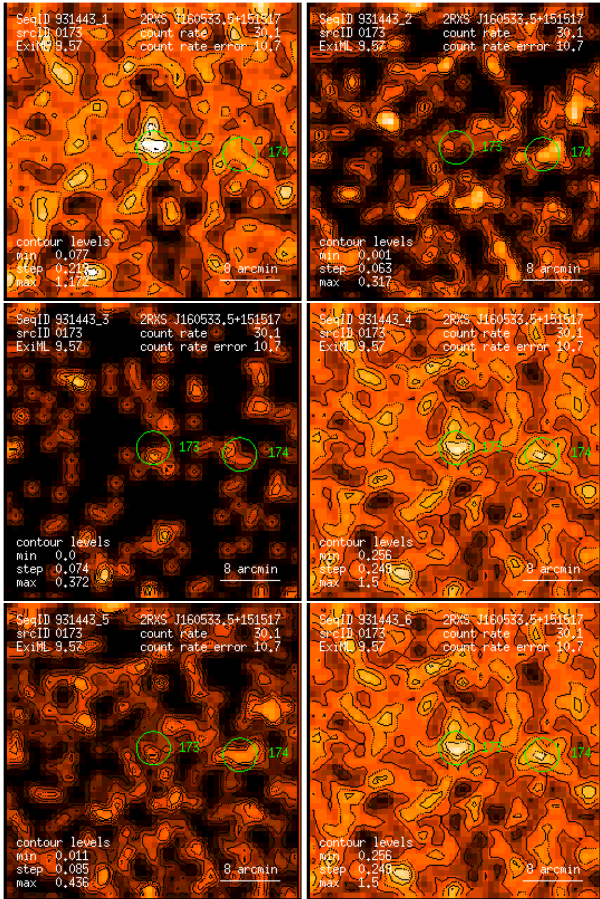
Figure 173: RASS 931443: detection 0173: band rate images, Gaussian filter: (1) PSPC channels 11 – 41, (2) 52 – 90, (3) 91 – 201, (4) 11 – 235, (5) 52 – 201, (6) 11 – 201. Broad band rates in counts/ks. Band rate contour levels in counts/ks/arcmin 2 .
