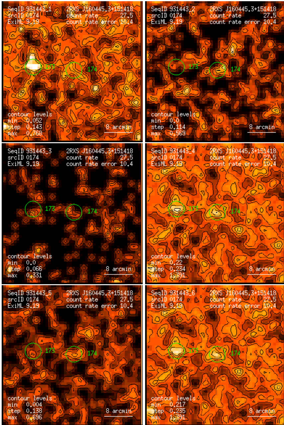
Figure 174: RASS 931443: detection 0174: band rate images, Gaussian filter: (1) PSPC channels 11 – 41, (2) 52 – 90, (3) 91 – 201, (4) 11 – 235, (5) 52 – 201, (6) 11 – 201. Broad band rates in counts/ks. Band rate contour levels in counts/ks/arcmin 2 .
