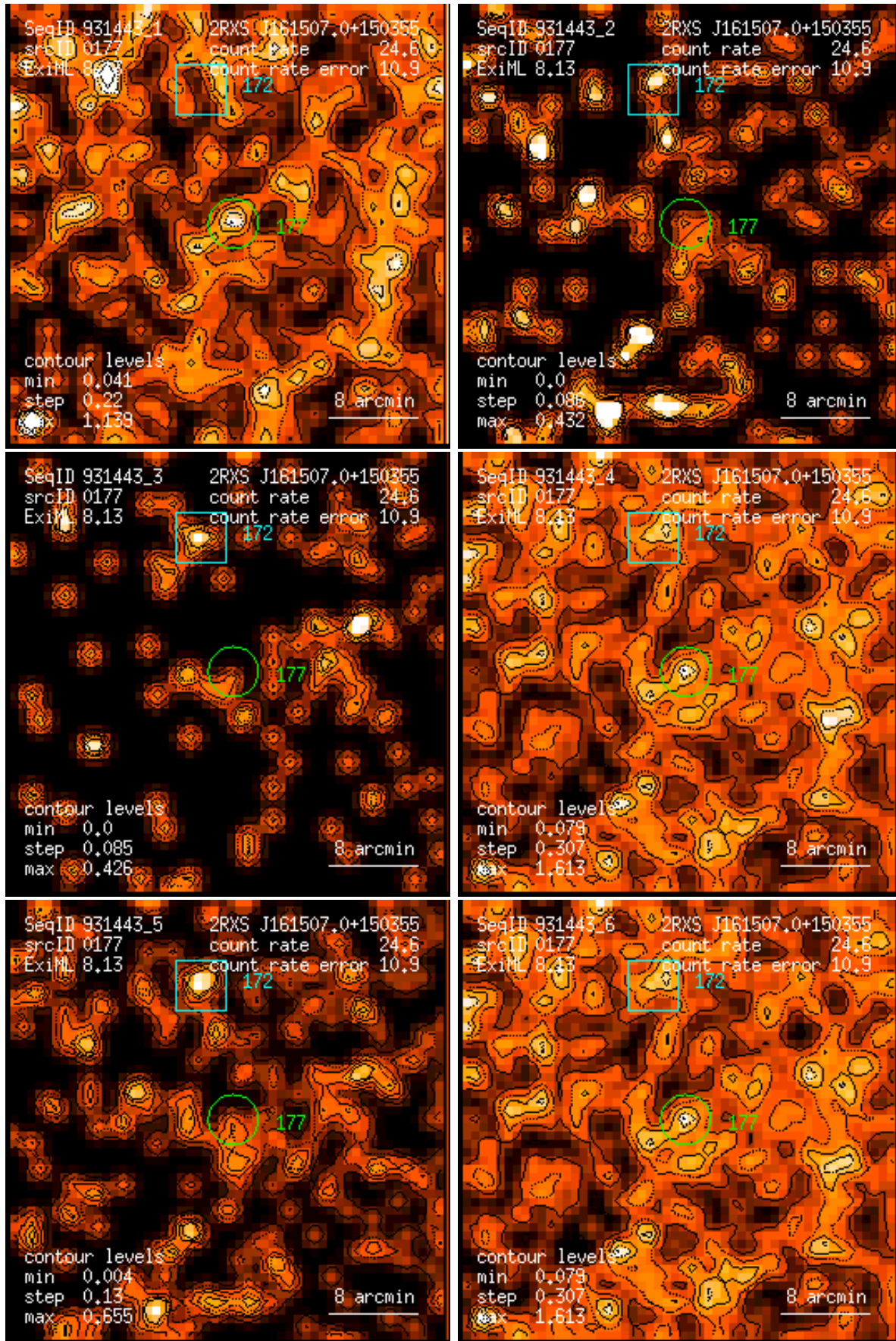
Figure 177: RASS 931443: detection 0177: band rate images, Gaussian filter: (1) PSPC channels 11 – 41, (2) 52 – 90, (3) 91 – 201, (4) 11 – 235, (5) 52 – 201, (6) 11 – 201. Broad band rates in counts/ks. Band rate contour levels in counts/ks/arcmin 2 .
