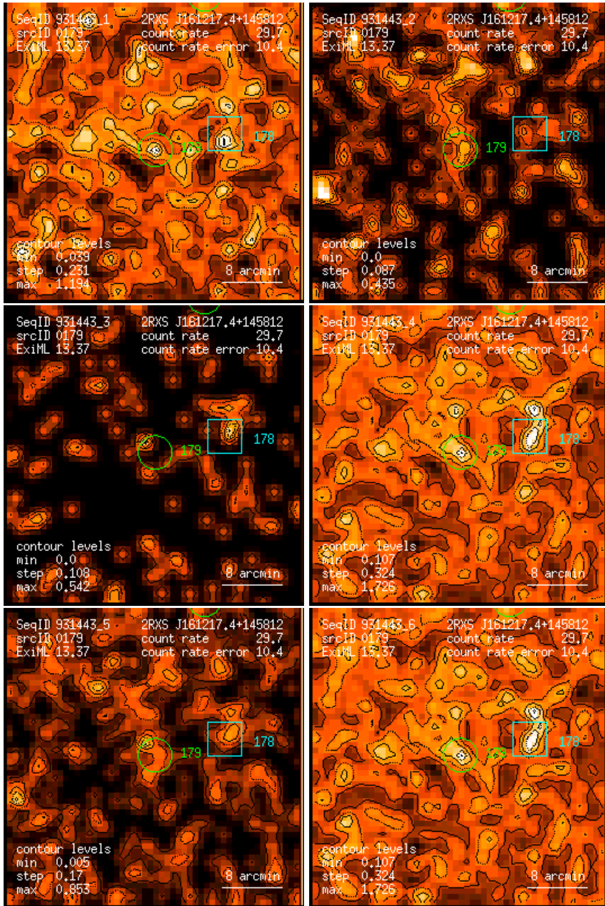
Figure 179: RASS 931443: detection 0179: band rate images, Gaussian filter: (1) PSPC channels 11 – 41, (2) 52 – 90, (3) 91 – 201, (4) 11 – 235, (5) 52 – 201, (6) 11 – 201. Broad band rates in counts/ks. Band rate contour levels in counts/ks/arcmin 2 .
