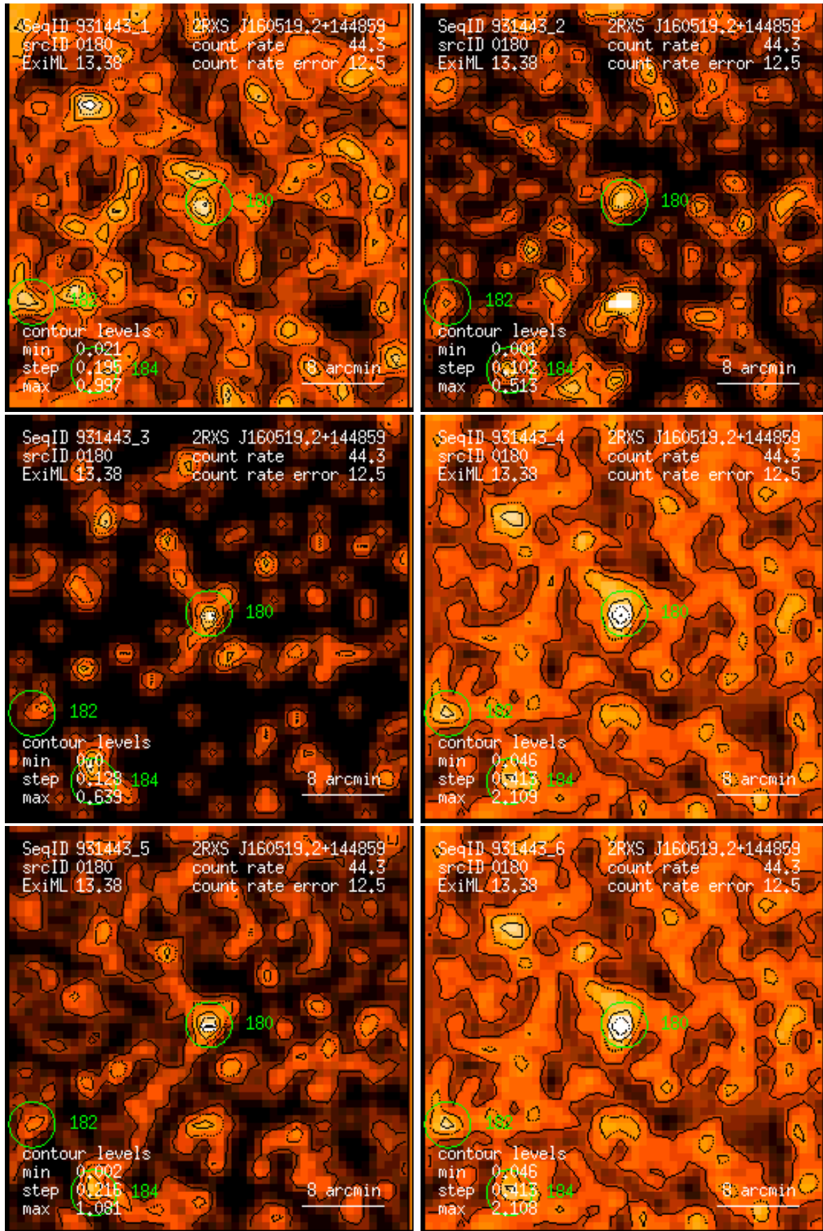
Figure 180: RASS 931443: detection 0180: band rate images, Gaussian filter: (1) PSPC channels 11 – 41, (2) 52 – 90, (3) 91 – 201, (4) 11 – 235, (5) 52 – 201, (6) 11 – 201. Broad band rates in counts/ks. Band rate contour levels in counts/ks/arcmin 2 .
