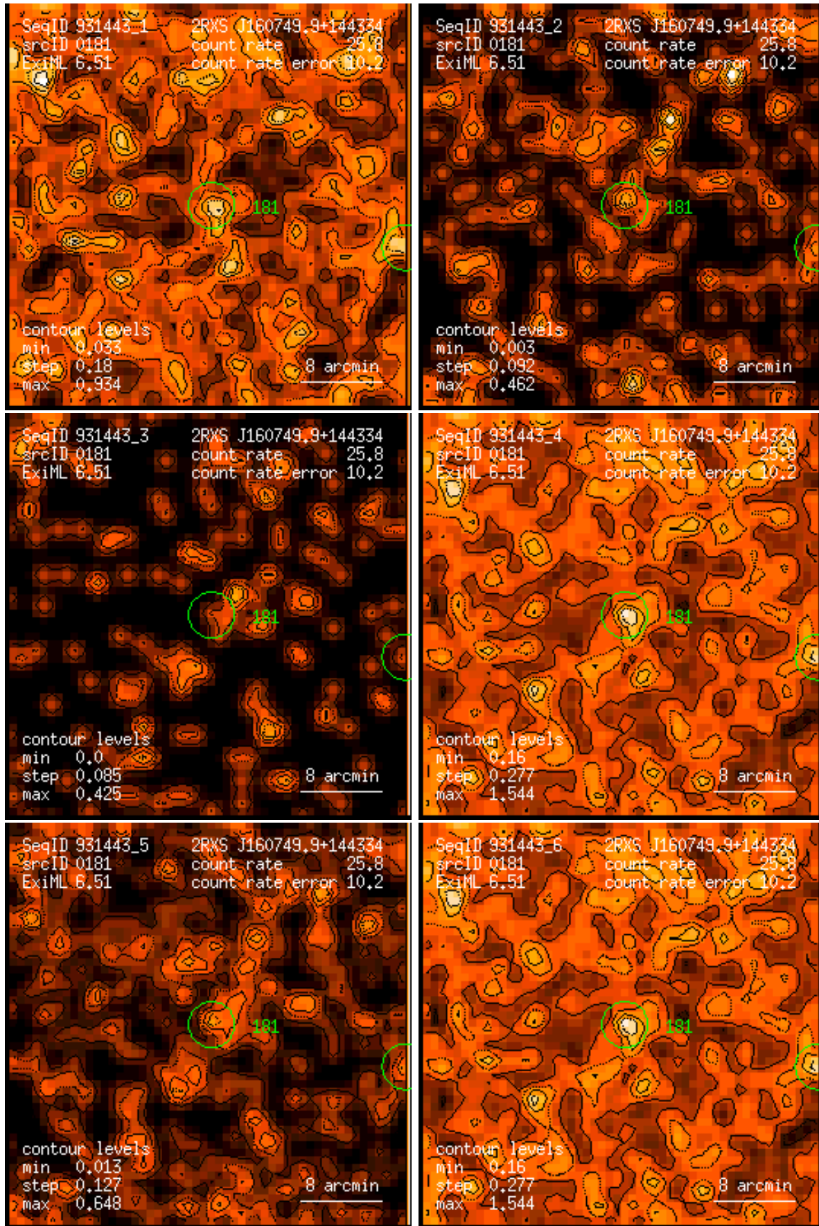
Figure 181: RASS 931443: detection 0181: band rate images, Gaussian filter: (1) PSPC channels 11 – 41, (2) 52 – 90, (3) 91 – 201, (4) 11 – 235, (5) 52 – 201, (6) 11 – 201. Broad band rates in counts/ks. Band rate contour levels in counts/ks/arcmin 2 .
