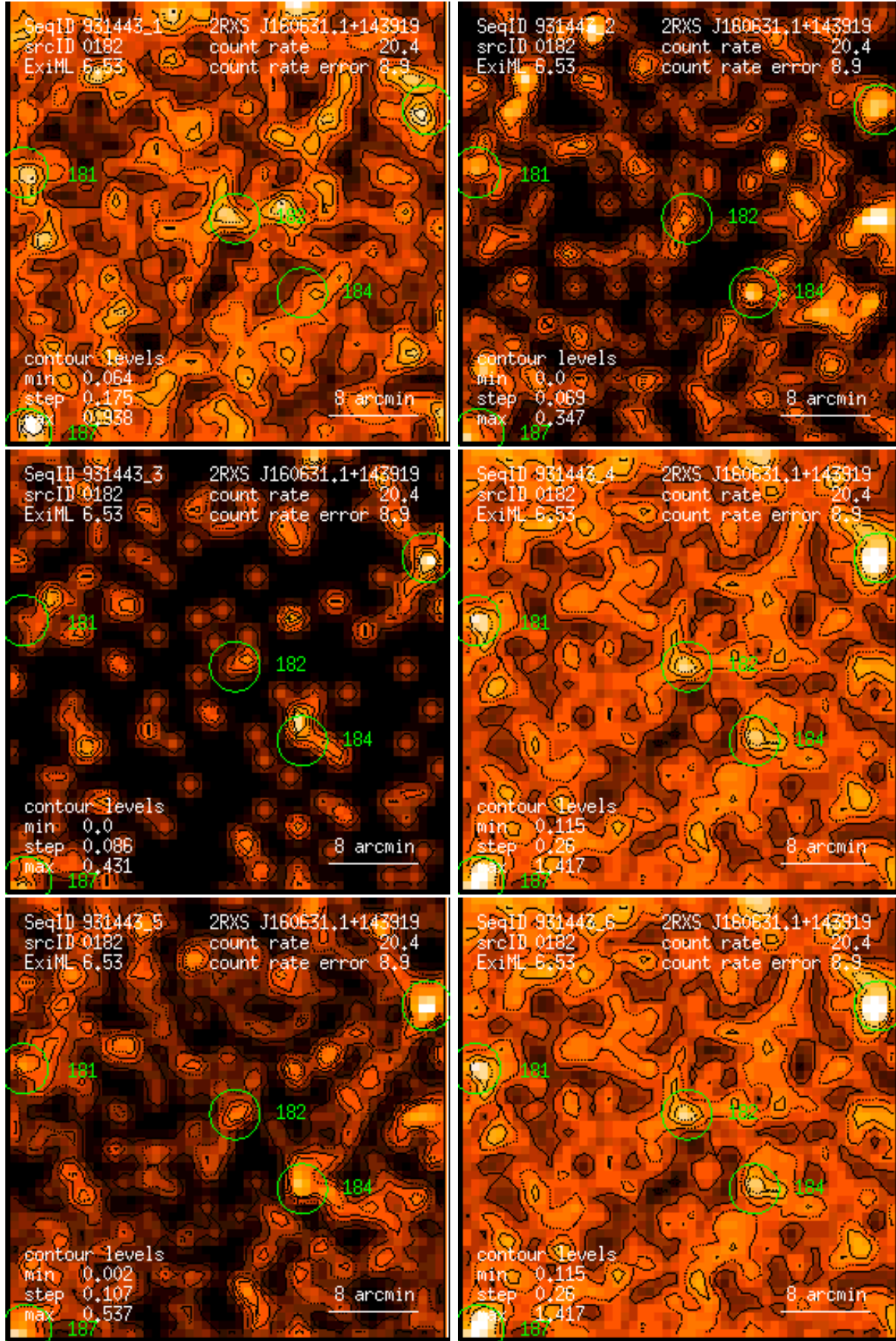
Figure 182: RASS 931443: detection 0182: band rate images, Gaussian filter: (1) PSPC channels 11 – 41, (2) 52 – 90, (3) 91 – 201, (4) 11 – 235, (5) 52 – 201, (6) 11 – 201. Broad band rates in counts/ks. Band rate contour levels in counts/ks/arcmin 2 .
