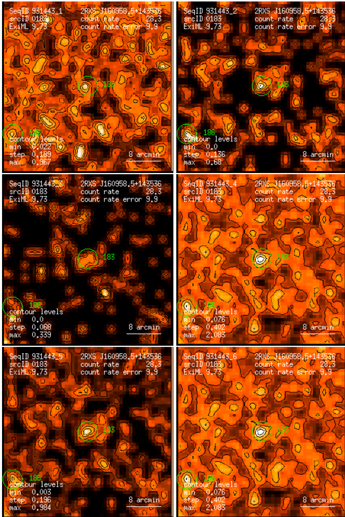
Figure 183: RASS 931443: detection 0183: band rate images, Gaussian filter: (1) PSPC channels 11 – 41, (2) 52 – 90, (3) 91 – 201, (4) 11 – 235, (5) 52 – 201, (6) 11 – 201. Broad band rates in counts/ks. Band rate contour levels in counts/ks/arcmin 2 .
