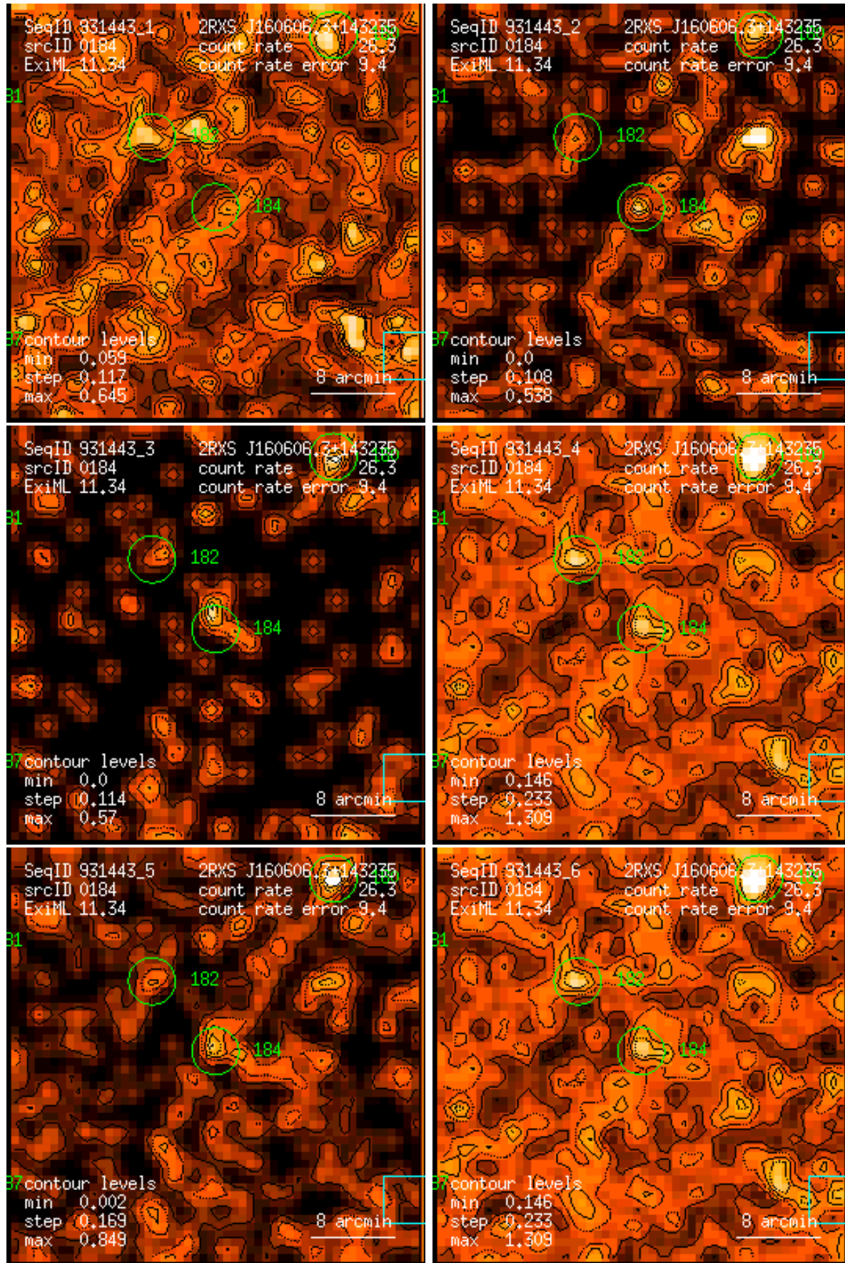
Figure 184: RASS 931443: detection 0184: band rate images, Gaussian filter: (1) PSPC channels 11 – 41, (2) 52 – 90, (3) 91 – 201, (4) 11 – 235, (5) 52 – 201, (6) 11 – 201. Broad band rates in counts/ks. Band rate contour levels in counts/ks/arcmin 2 .
