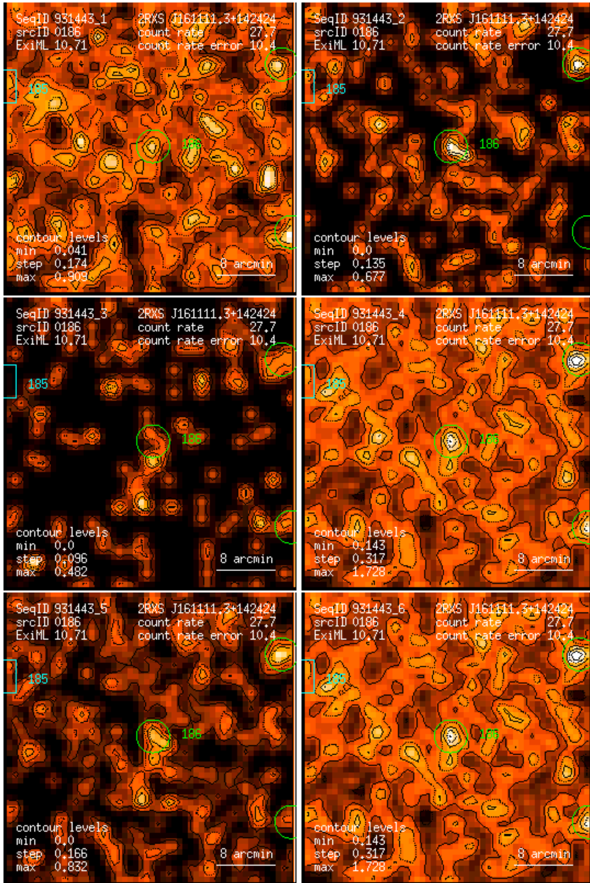
Figure 186: RASS 931443: detection 0186: band rate images, Gaussian filter: (1) PSPC channels 11 – 41, (2) 52 – 90, (3) 91 – 201, (4) 11 – 235, (5) 52 – 201, (6) 11 – 201. Broad band rates in counts/ks. Band rate contour levels in counts/ks/arcmin 2 .
