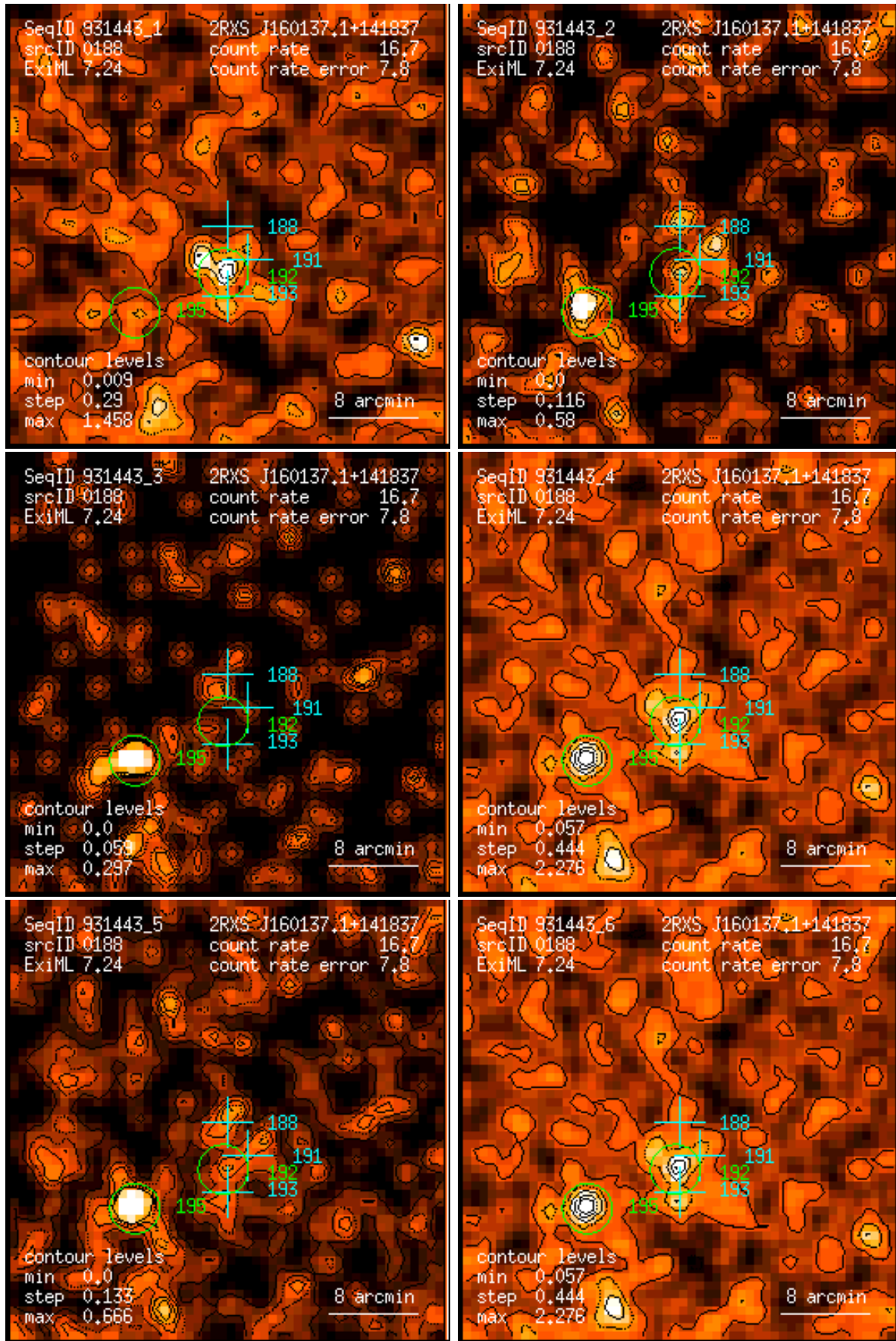
Figure 188: RASS 931443: detection 0188: band rate images, Gaussian filter: (1) PSPC channels 11 – 41, (2) 52 – 90, (3) 91 – 201, (4) 11 – 235, (5) 52 – 201, (6) 11 – 201. Broad band rates in counts/ks. Band rate contour levels in counts/ks/arcmin 2 .
