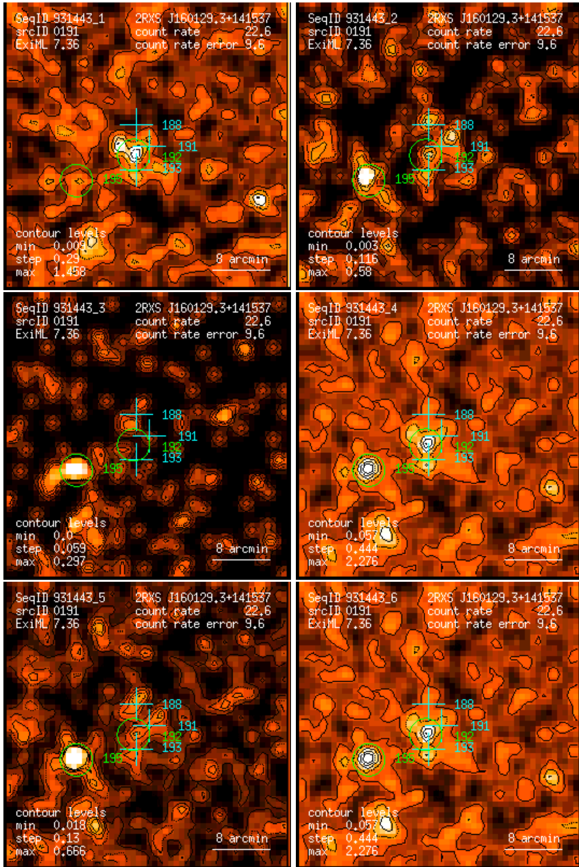
Figure 191: RASS 931443: detection 0191: band rate images, Gaussian filter: (1) PSPC channels 11 – 41, (2) 52 – 90, (3) 91 – 201, (4) 11 – 235, (5) 52 – 201, (6) 11 – 201. Broad band rates in counts/ks. Band rate contour levels in counts/ks/arcmin 2 .
