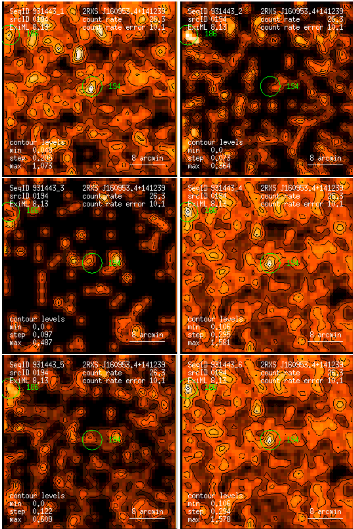
Figure 194: RASS 931443: detection 0194: band rate images, Gaussian filter: (1) PSPC channels 11 – 41, (2) 52 – 90, (3) 91 – 201, (4) 11 – 235, (5) 52 – 201, (6) 11 – 201. Broad band rates in counts/ks. Band rate contour levels in counts/ks/arcmin 2 .
