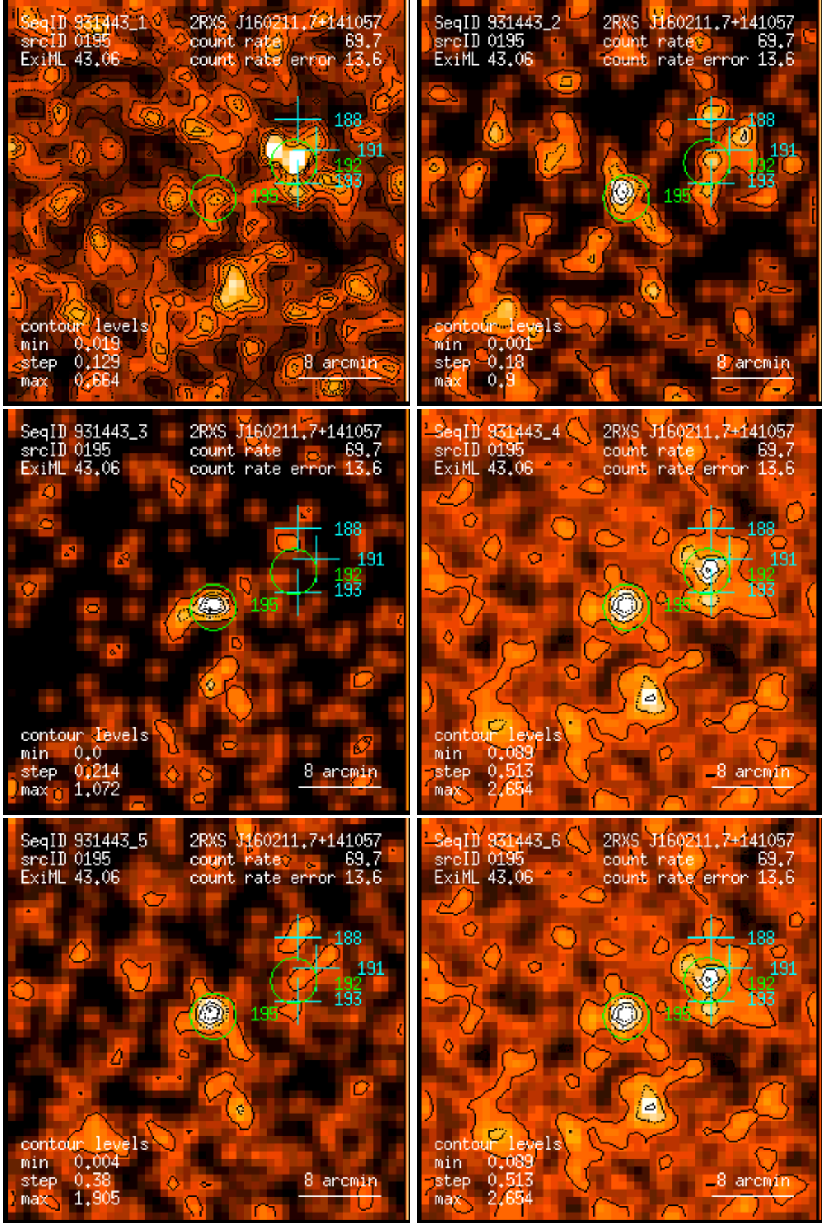
Figure 195: RASS 931443: detection 0195: band rate images, Gaussian filter: (1) PSPC channels 11 – 41, (2) 52 – 90, (3) 91 – 201, (4) 11 – 235, (5) 52 – 201, (6) 11 – 201. Broad band rates in counts/ks. Band rate contour levels in counts/ks/arcmin 2 .
