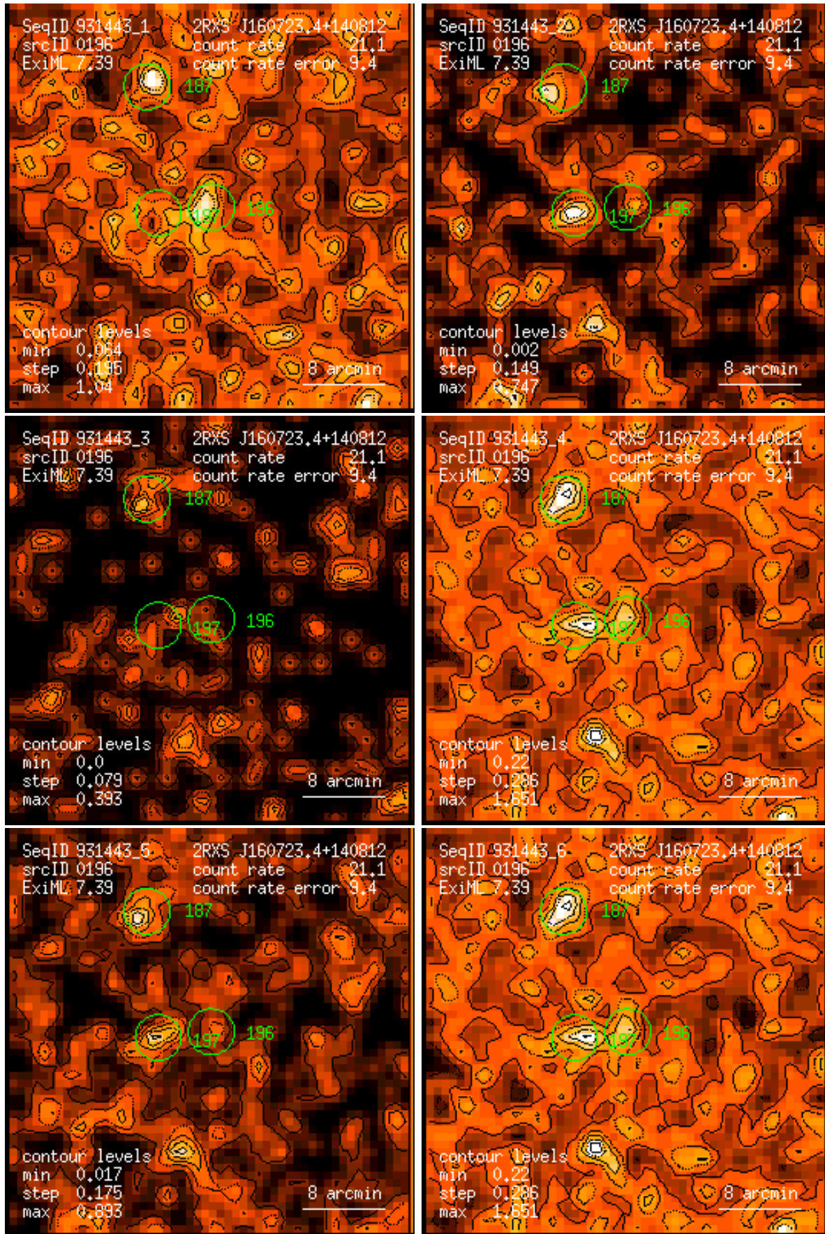
Figure 196: RASS 931443: detection 0196: band rate images, Gaussian filter: (1) PSPC channels 11 – 41, (2) 52 – 90, (3) 91 – 201, (4) 11 – 235, (5) 52 – 201, (6) 11 – 201. Broad band rates in counts/ks. Band rate contour levels in counts/ks/arcmin 2 .
