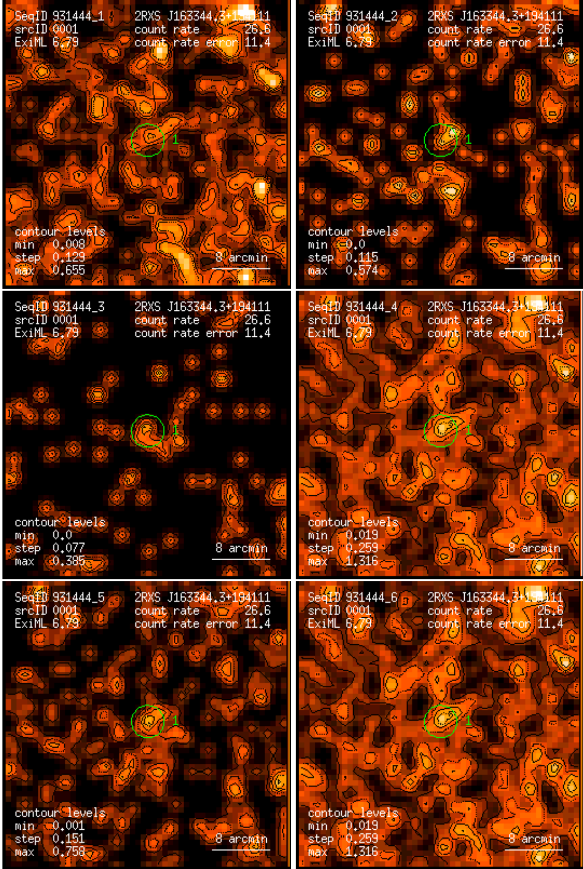
Figure 1: RASS 931444: detection 0001: band rate images, Gaussian filter: (1) PSPC channels 11 – 41, (2) 52 – 90, (3) 91 – 201, (4) 11 – 235, (5) 52 – 201, (6) 11 – 201. Broad band rates in counts/ks. Band rate contour levels in counts/ks/arcmin 2 .
