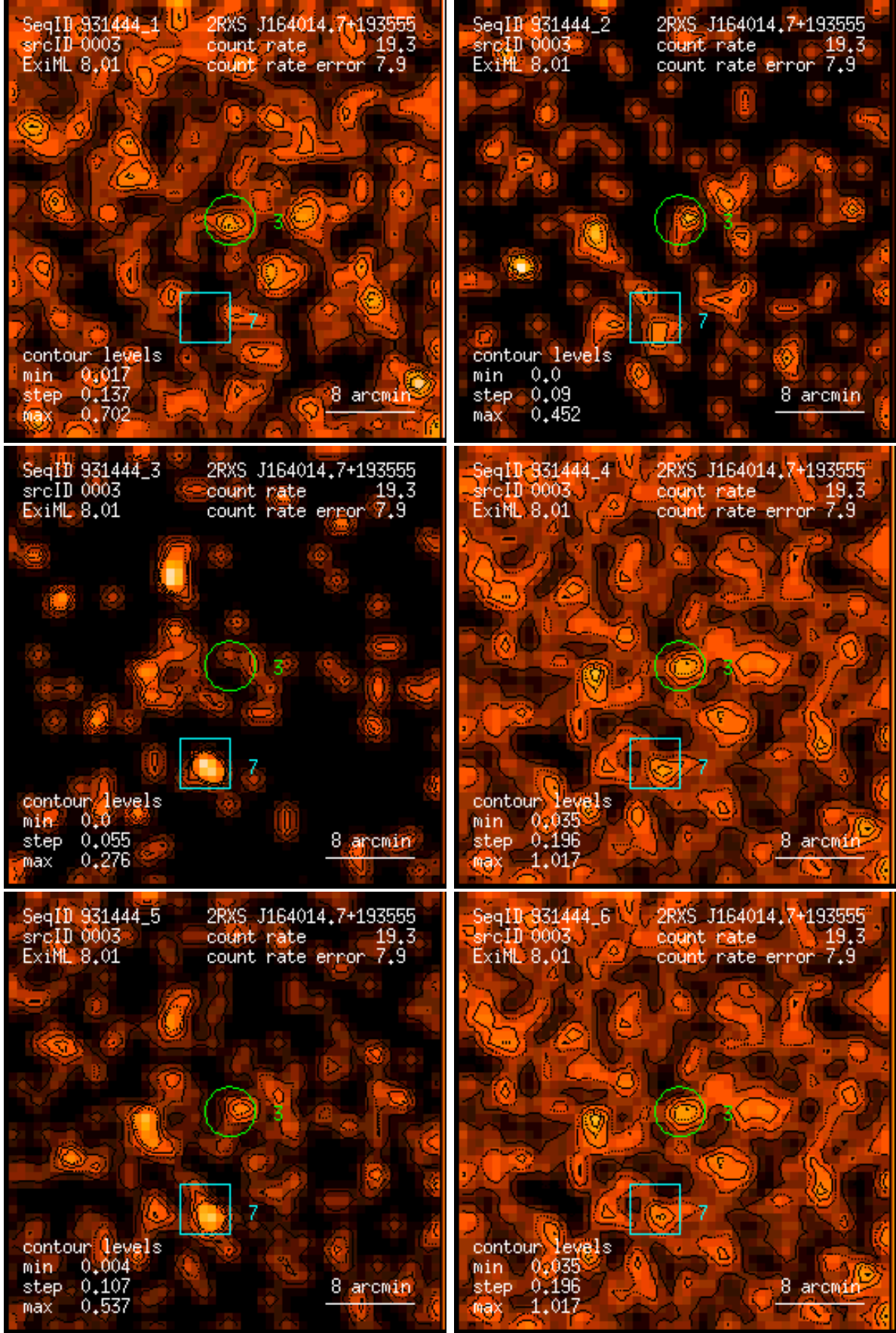
Figure 3: RASS 931444: detection 0003: band rate images, Gaussian filter: (1) PSPC channels 11 – 41, (2) 52 – 90, (3) 91 – 201, (4) 11 – 235, (5) 52 – 201, (6) 11 – 201. Broad band rates in counts/ks. Band rate contour levels in counts/ks/arcmin 2 .
