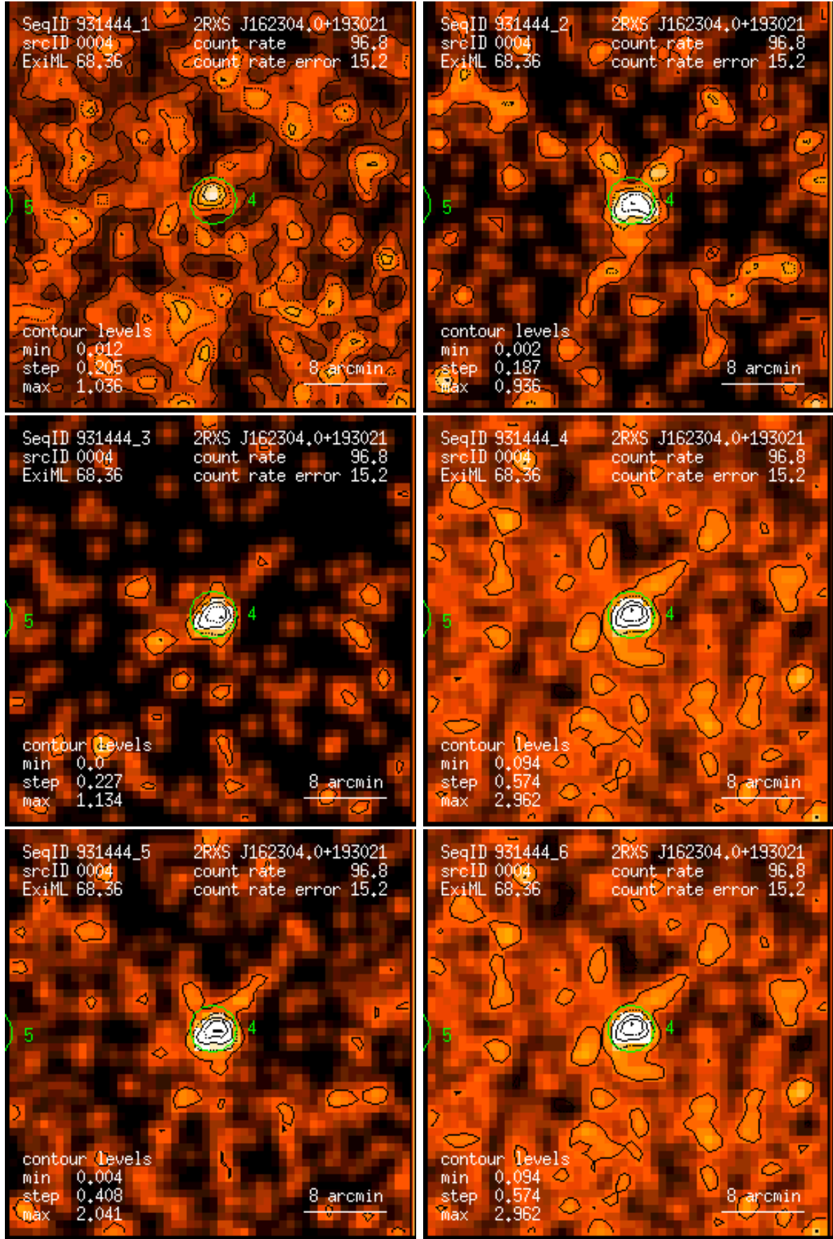
Figure 4: RASS 931444: detection 0004: band rate images, Gaussian filter: (1) PSPC channels 11 – 41, (2) 52 – 90, (3) 91 – 201, (4) 11 – 235, (5) 52 – 201, (6) 11 – 201. Broad band rates in counts/ks. Band rate contour levels in counts/ks/arcmin 2 .
