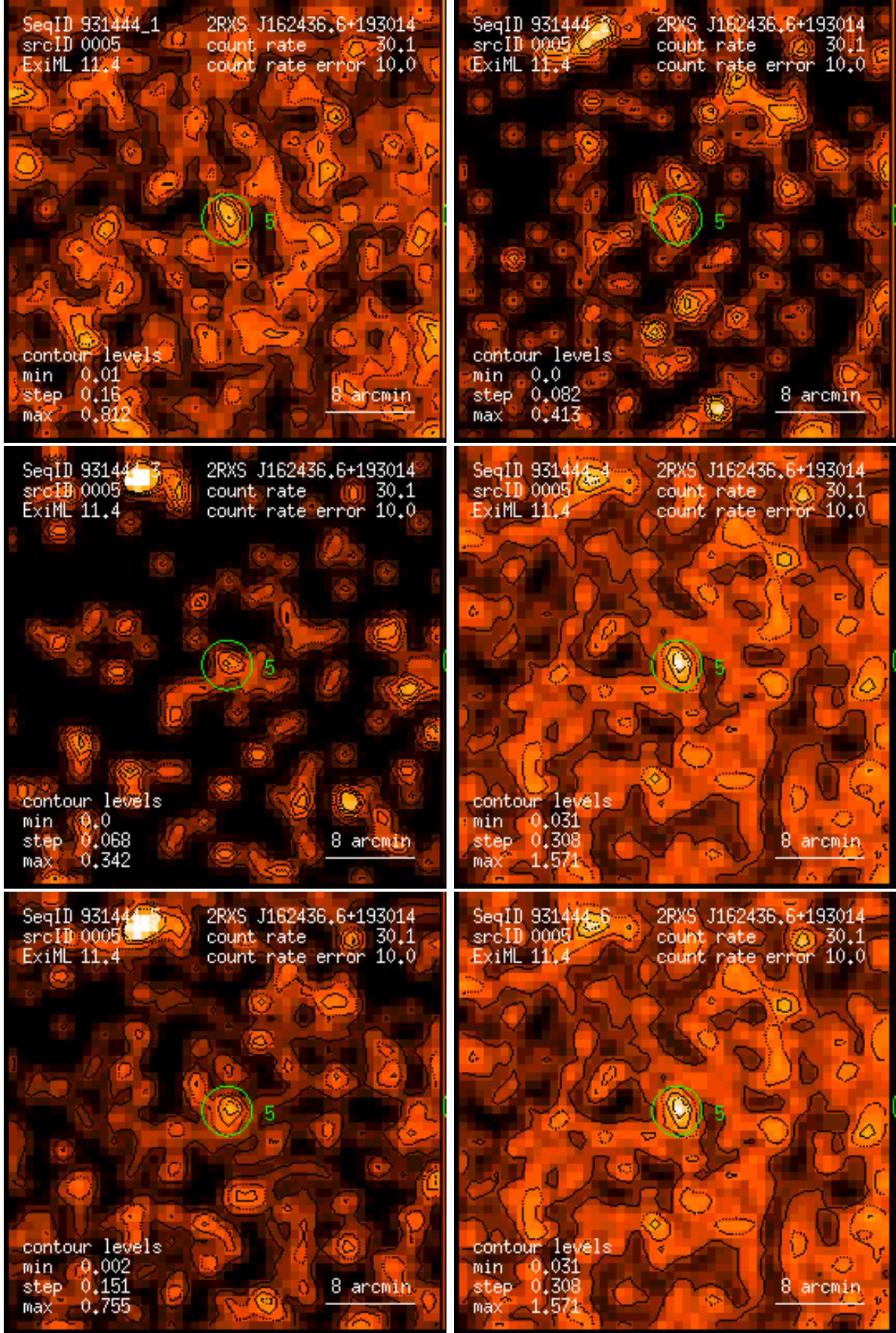
Figure 5: RASS 931444: detection 0005: band rate images, Gaussian filter: (1) PSPC channels 11 – 41, (2) 52 – 90, (3) 91 – 201, (4) 11 – 235, (5) 52 – 201, (6) 11 – 201. Broad band rates in counts/ks. Band rate contour levels in counts/ks/arcmin 2 .
