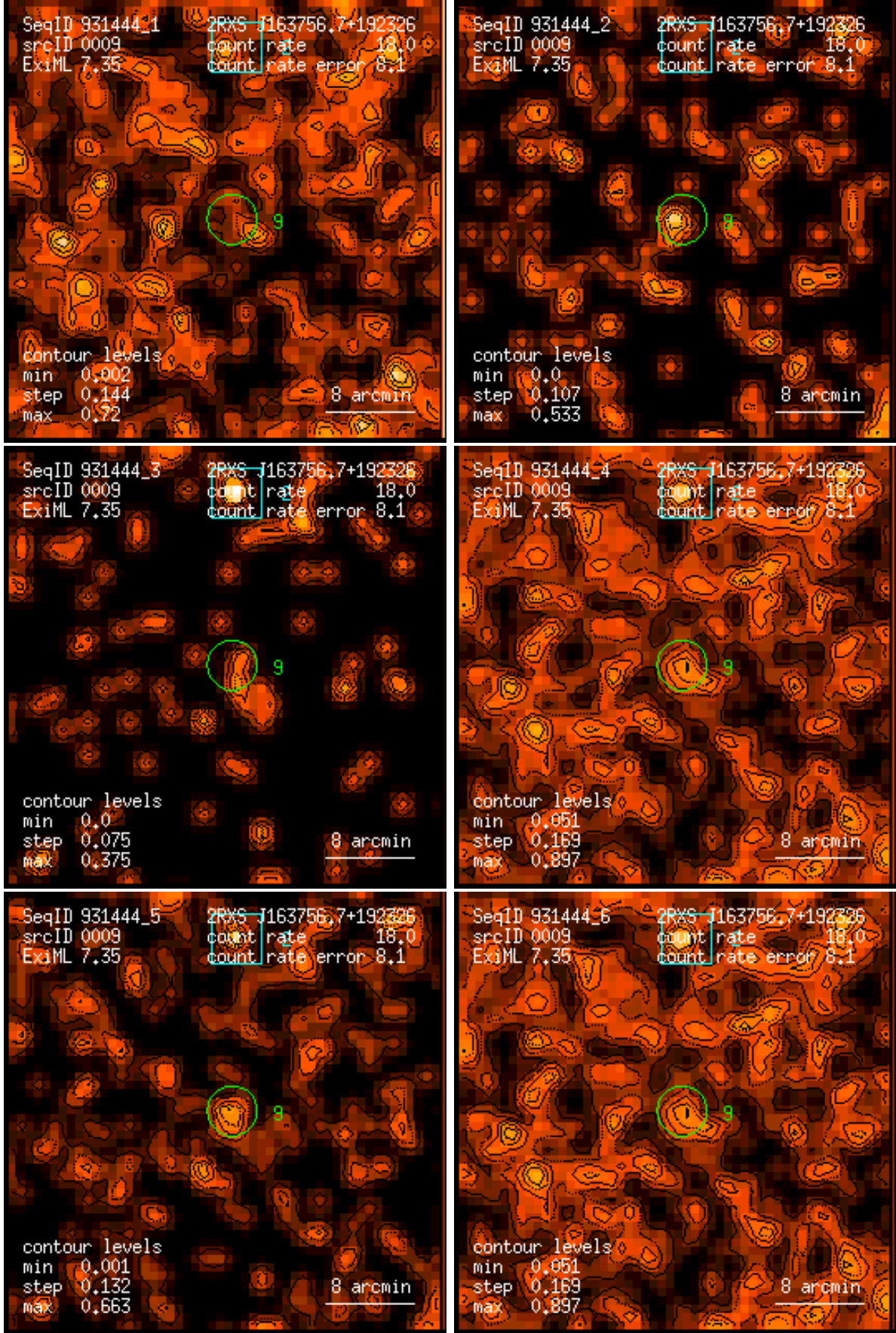
Figure 9: RASS 931444: detection 0009: band rate images, Gaussian filter: (1) PSPC channels 11 – 41, (2) 52 – 90, (3) 91 – 201, (4) 11 – 235, (5) 52 – 201, (6) 11 – 201. Broad band rates in counts/ks. Band rate contour levels in counts/ks/arcmin 2 .
