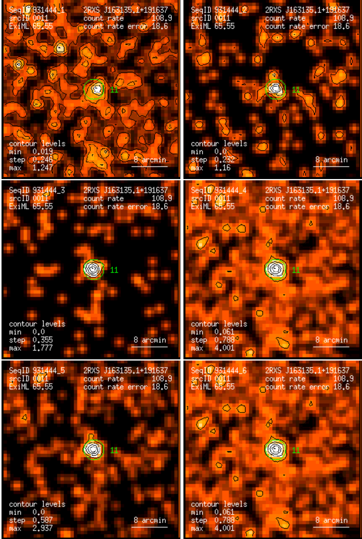
Figure 11: RASS 931444: detection 0011: band rate images, Gaussian filter: (1) PSPC channels 11 – 41, (2) 52 – 90, (3) 91 – 201, (4) 11 – 235, (5) 52 – 201, (6) 11 – 201. Broad band rates in counts/ks. Band rate contour levels in counts/ks/arcmin 2 .
