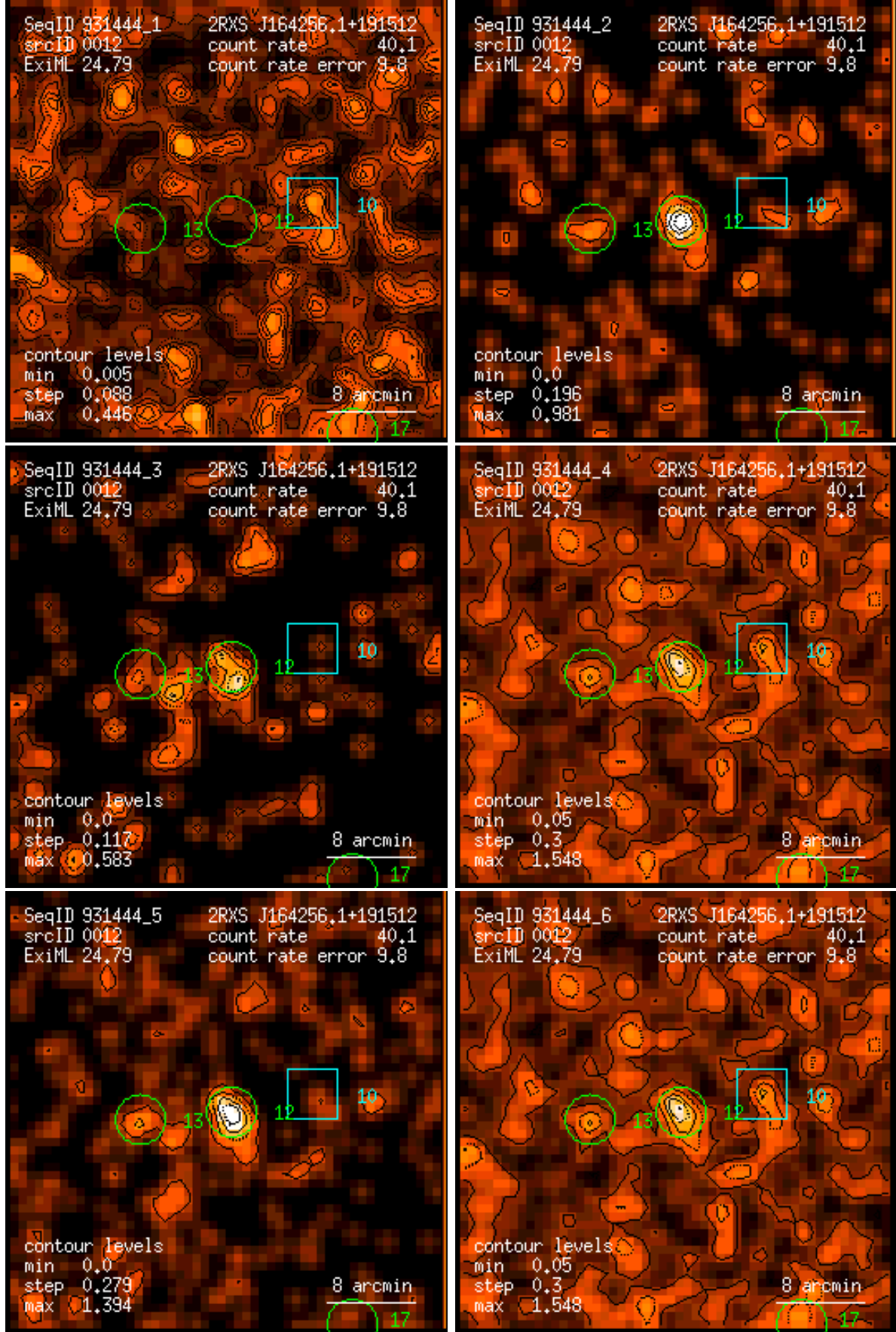
Figure 12: RASS 931444: detection 0012: band rate images, Gaussian filter: (1) PSPC channels 11 – 41, (2) 52 – 90, (3) 91 – 201, (4) 11 – 235, (5) 52 – 201, (6) 11 – 201. Broad band rates in counts/ks. Band rate contour levels in counts/ks/arcmin 2 .
