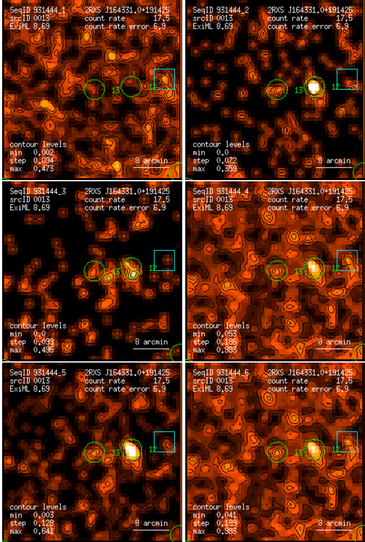
Figure 13: RASS 931444: detection 0013: band rate images, Gaussian filter: (1) PSPC channels 11 – 41, (2) 52 – 90, (3) 91 – 201, (4) 11 – 235, (5) 52 – 201, (6) 11 – 201. Broad band rates in counts/ks. Band rate contour levels in counts/ks/arcmin 2 .
