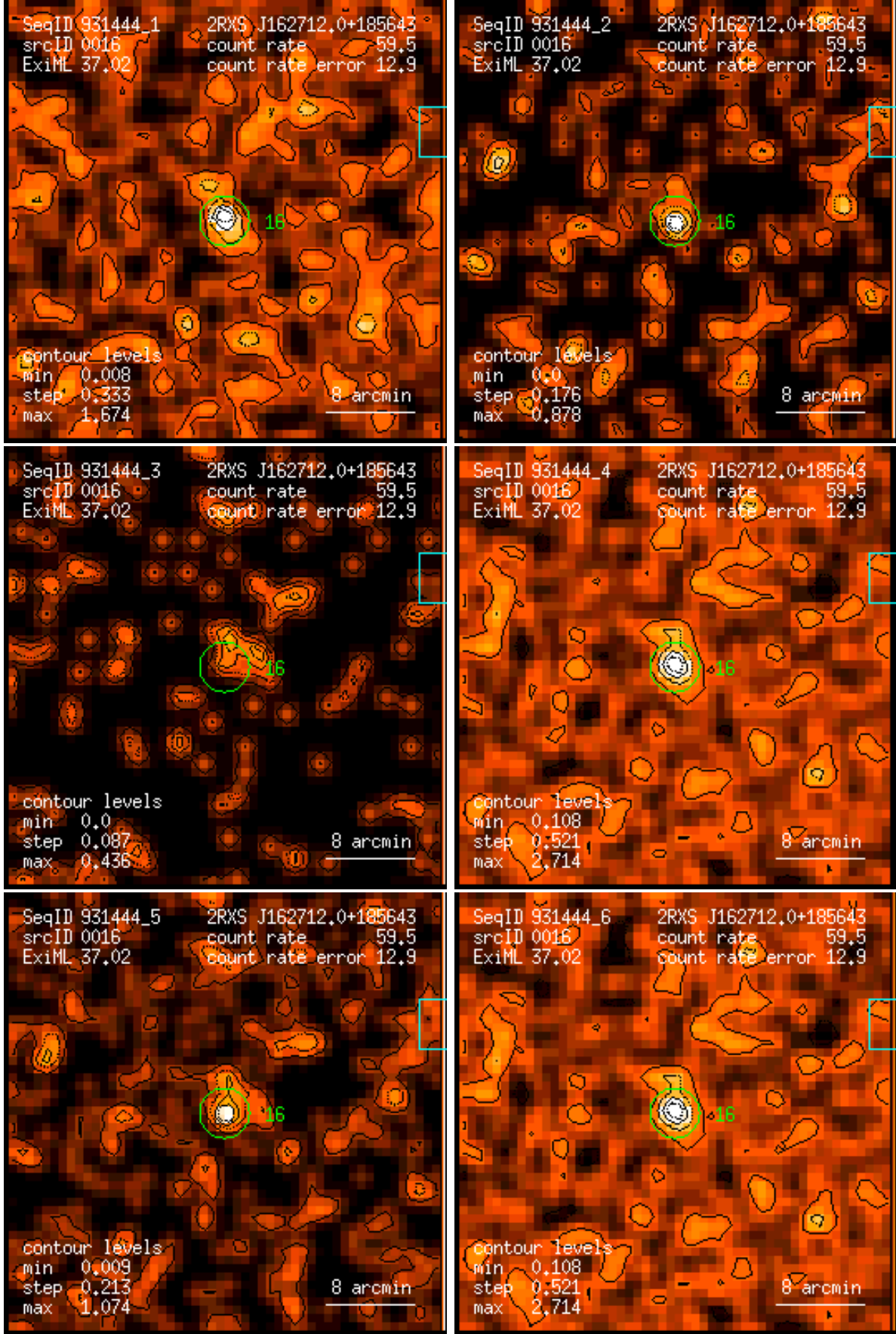
Figure 16: RASS 931444: detection 0016: band rate images, Gaussian filter: (1) PSPC channels 11 – 41, (2) 52 – 90, (3) 91 – 201, (4) 11 – 235, (5) 52 – 201, (6) 11 – 201. Broad band rates in counts/ks. Band rate contour levels in counts/ks/arcmin 2 .
