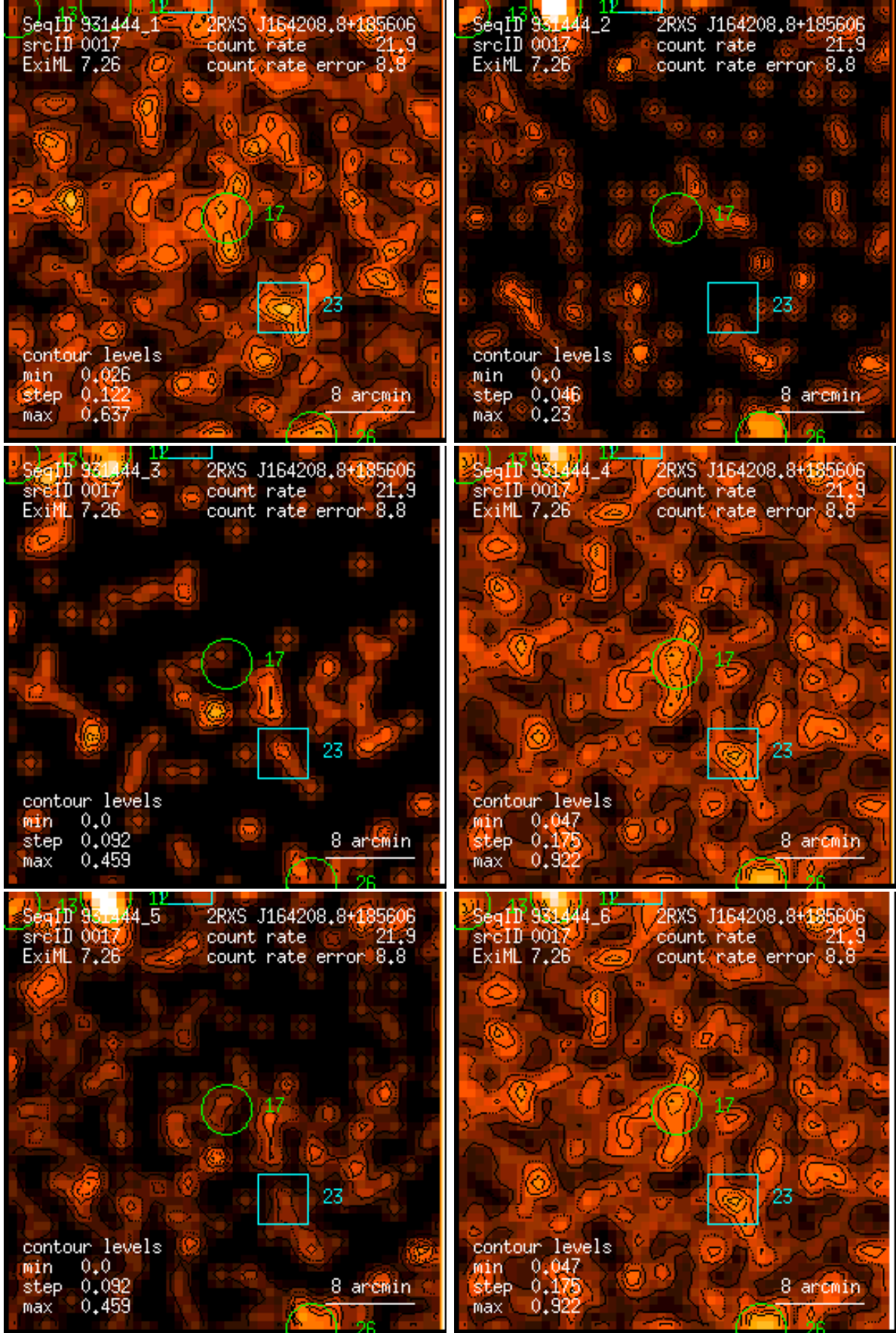
Figure 17: RASS 931444: detection 0017: band rate images, Gaussian filter: (1) PSPC channels 11 – 41, (2) 52 – 90, (3) 91 – 201, (4) 11 – 235, (5) 52 – 201, (6) 11 – 201. Broad band rates in counts/ks. Band rate contour levels in counts/ks/arcmin 2 .
