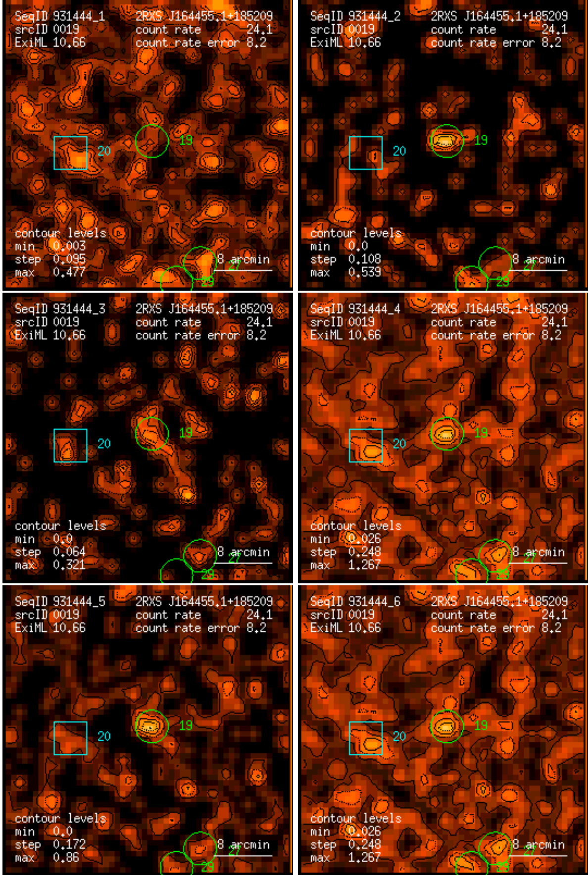
Figure 19: RASS 931444: detection 0019: band rate images, Gaussian filter: (1) PSPC channels 11 – 41, (2) 52 – 90, (3) 91 – 201, (4) 11 – 235, (5) 52 – 201, (6) 11 – 201. Broad band rates in counts/ks. Band rate contour levels in counts/ks/arcmin 2 .
