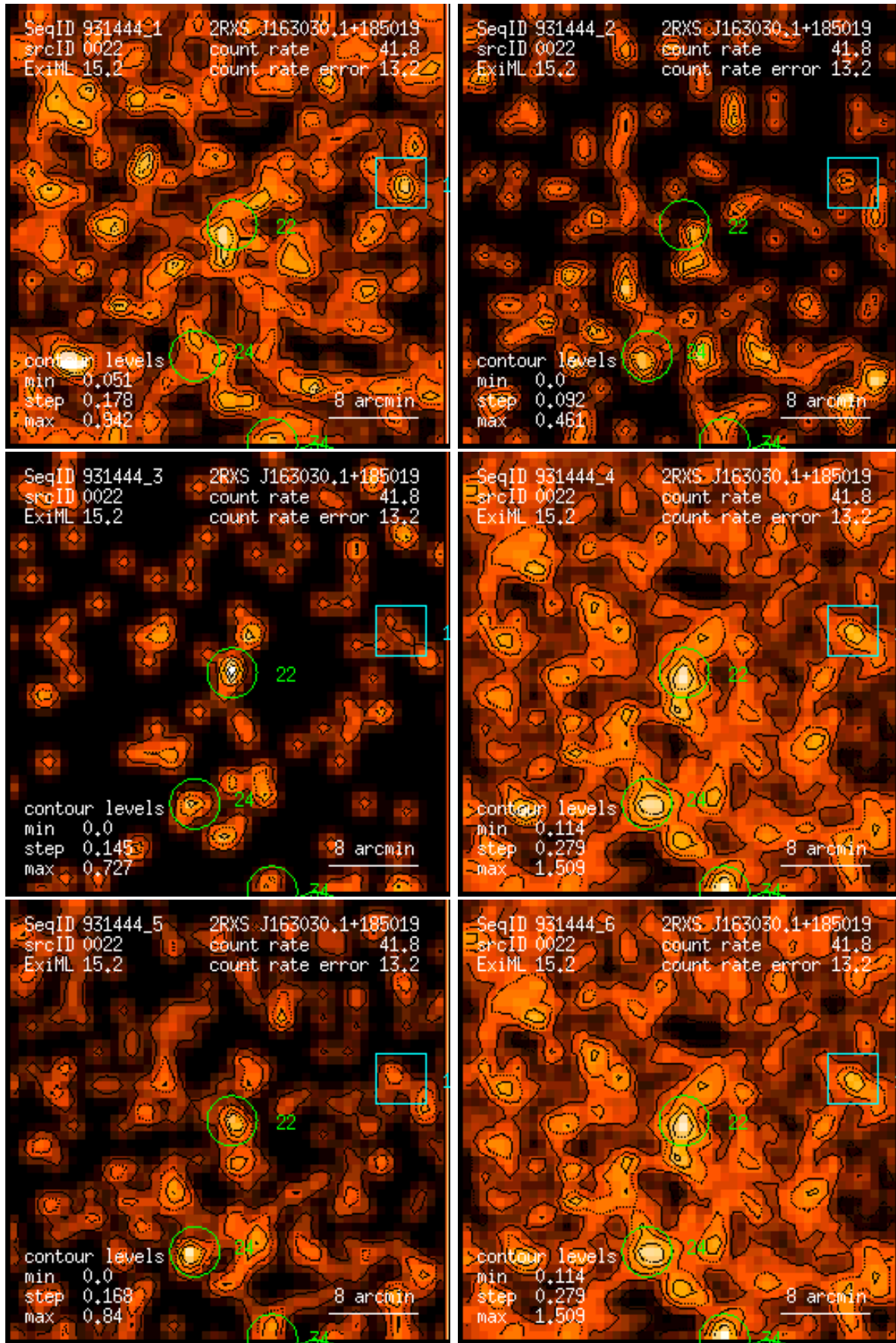
Figure 22: RASS 931444: detection 0022: band rate images, Gaussian filter: (1) PSPC channels 11 – 41, (2) 52 – 90, (3) 91 – 201, (4) 11 – 235, (5) 52 – 201, (6) 11 – 201. Broad band rates in counts/ks. Band rate contour levels in counts/ks/arcmin 2 .
