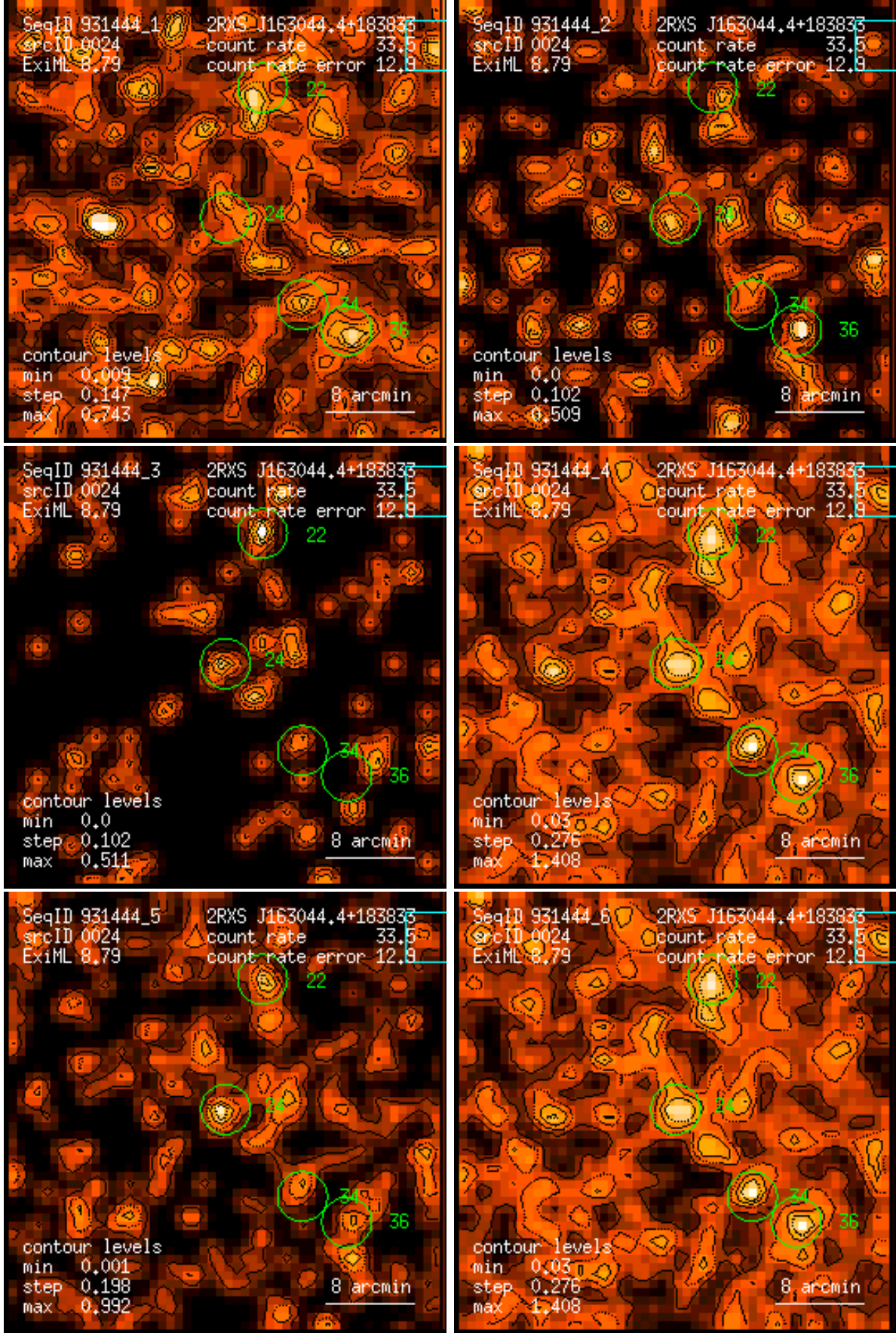
Figure 24: RASS 931444: detection 0024: band rate images, Gaussian filter: (1) PSPC channels 11 – 41, (2) 52 – 90, (3) 91 – 201, (4) 11 – 235, (5) 52 – 201, (6) 11 – 201. Broad band rates in counts/ks. Band rate contour levels in counts/ks/arcmin 2 .
