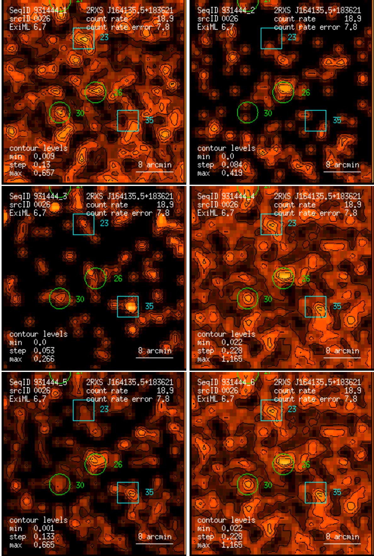
Figure 26: RASS 931444: detection 0026: band rate images, Gaussian filter: (1) PSPC channels 11 – 41, (2) 52 – 90, (3) 91 – 201, (4) 11 – 235, (5) 52 – 201, (6) 11 – 201. Broad band rates in counts/ks. Band rate contour levels in counts/ks/arcmin 2 .
