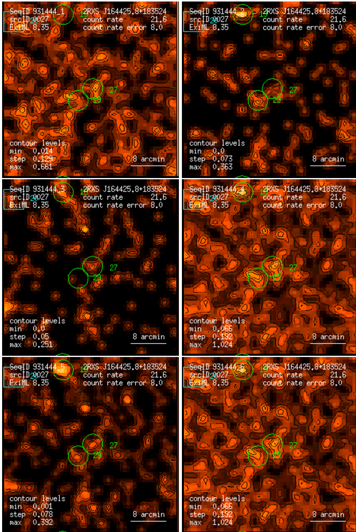
Figure 27: RASS 931444: detection 0027: band rate images, Gaussian filter: (1) PSPC channels 11 – 41, (2) 52 – 90, (3) 91 – 201, (4) 11 – 235, (5) 52 – 201, (6) 11 – 201. Broad band rates in counts/ks. Band rate contour levels in counts/ks/arcmin 2 .
