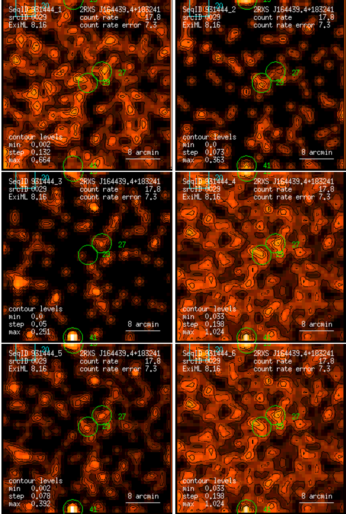
Figure 29: RASS 931444: detection 0029: band rate images, Gaussian filter: (1) PSPC channels 11 – 41, (2) 52 – 90, (3) 91 – 201, (4) 11 – 235, (5) 52 – 201, (6) 11 – 201. Broad band rates in counts/ks. Band rate contour levels in counts/ks/arcmin 2 .
