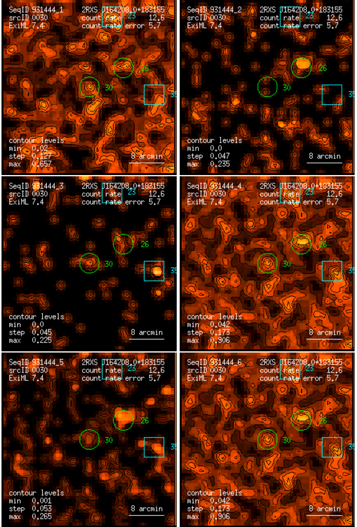
Figure 30: RASS 931444: detection 0030: band rate images, Gaussian filter: (1) PSPC channels 11 – 41, (2) 52 – 90, (3) 91 – 201, (4) 11 – 235, (5) 52 – 201, (6) 11 – 201. Broad band rates in counts/ks. Band rate contour levels in counts/ks/arcmin 2 .
