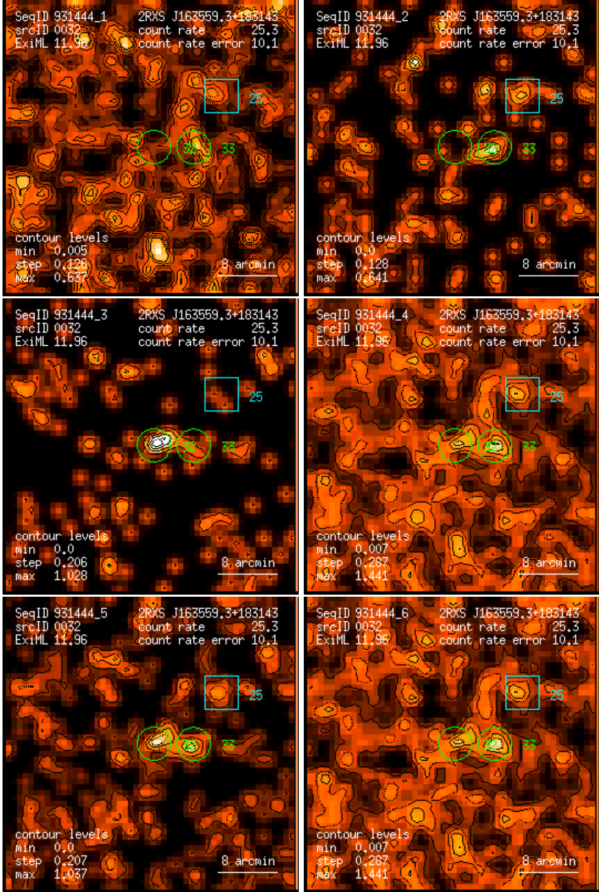
Figure 32: RASS 931444: detection 0032: band rate images, Gaussian filter: (1) PSPC channels 11 – 41, (2) 52 – 90, (3) 91 – 201, (4) 11 – 235, (5) 52 – 201, (6) 11 – 201. Broad band rates in counts/ks. Band rate contour levels in counts/ks/arcmin 2 .
