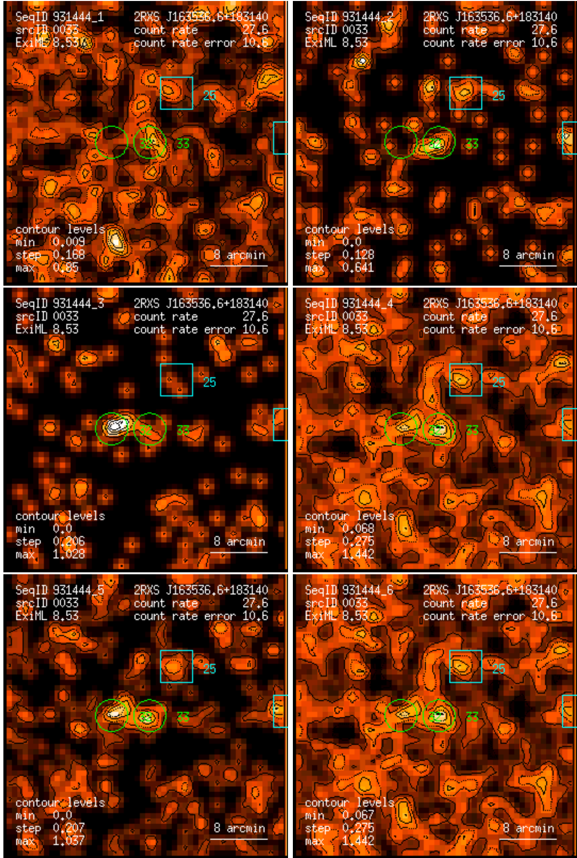
Figure 33: RASS 931444: detection 0033: band rate images, Gaussian filter: (1) PSPC channels 11 – 41, (2) 52 – 90, (3) 91 – 201, (4) 11 – 235, (5) 52 – 201, (6) 11 – 201. Broad band rates in counts/ks. Band rate contour levels in counts/ks/arcmin 2 .
