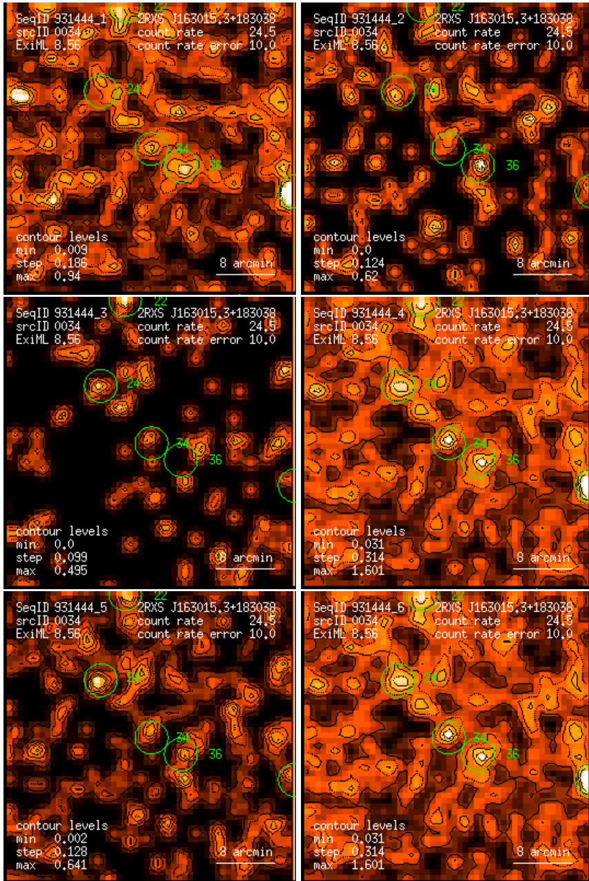
Figure 34: RASS 931444: detection 0034: band rate images, Gaussian filter: (1) PSPC channels 11 – 41, (2) 52 – 90, (3) 91 – 201, (4) 11 – 235, (5) 52 – 201, (6) 11 – 201. Broad band rates in counts/ks. Band rate contour levels in counts/ks/arcmin 2 .
