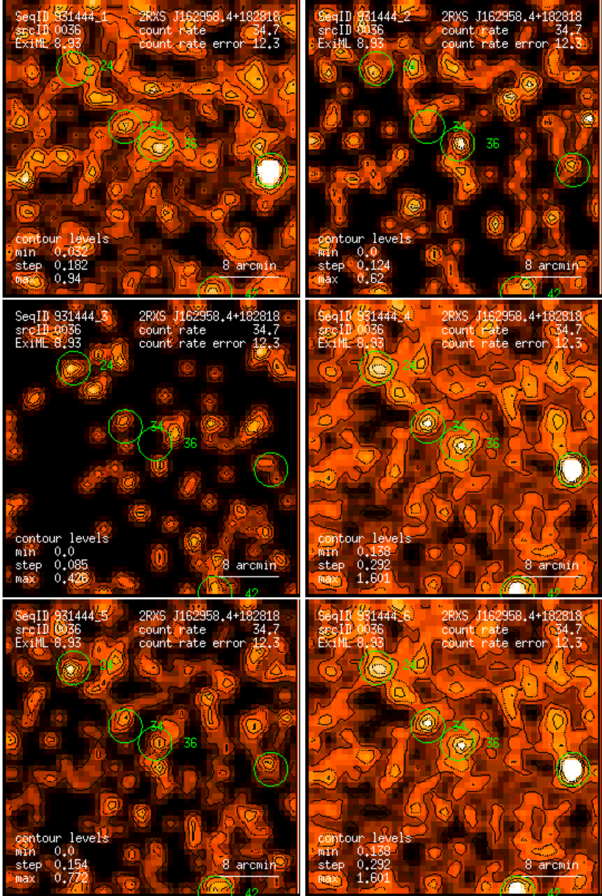
Figure 36: RASS 931444: detection 0036: band rate images, Gaussian filter: (1) PSPC channels 11 – 41, (2) 52 – 90, (3) 91 – 201, (4) 11 – 235, (5) 52 – 201, (6) 11 – 201. Broad band rates in counts/ks. Band rate contour levels in counts/ks/arcmin 2 .
