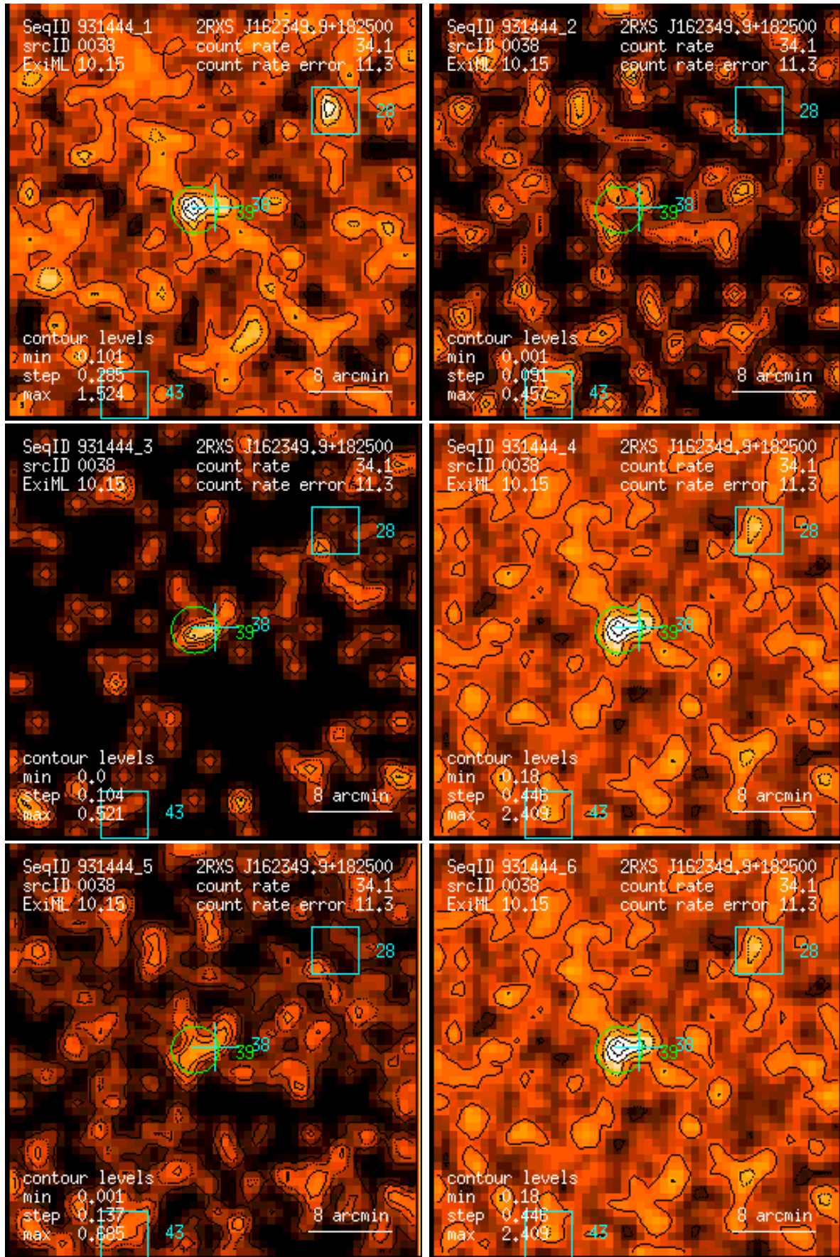
Figure 38: RASS 931444: detection 0038: band rate images, Gaussian filter: (1) PSPC channels 11 – 41, (2) 52 – 90, (3) 91 – 201, (4) 11 – 235, (5) 52 – 201, (6) 11 – 201. Broad band rates in counts/ks. Band rate contour levels in counts/ks/arcmin 2 .
