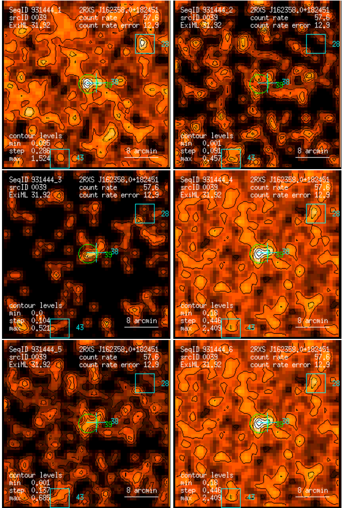
Figure 39: RASS 931444: detection 0039: band rate images, Gaussian filter: (1) PSPC channels 11 – 41, (2) 52 – 90, (3) 91 – 201, (4) 11 – 235, (5) 52 – 201, (6) 11 – 201. Broad band rates in counts/ks. Band rate contour levels in counts/ks/arcmin 2 .
